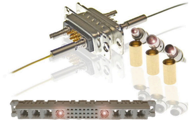
EBOSA™ termini in a D-sub DIN-41652 connector and DIN-41612 backplane connector.
