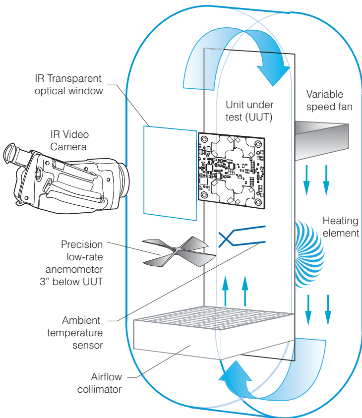
Figure 8. Vertical Wind Tunnel
