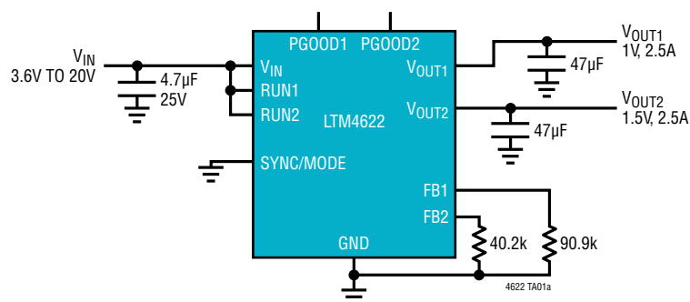
μModule Solution (LTM4622 Demo Circuit 2249B Dual 2.5A Output)
