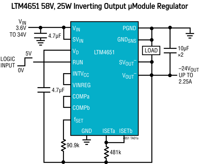
LTM4651 Can Be Driven by Typical Logic Level Signals. Does Not Require Level-Shift Circuitry
