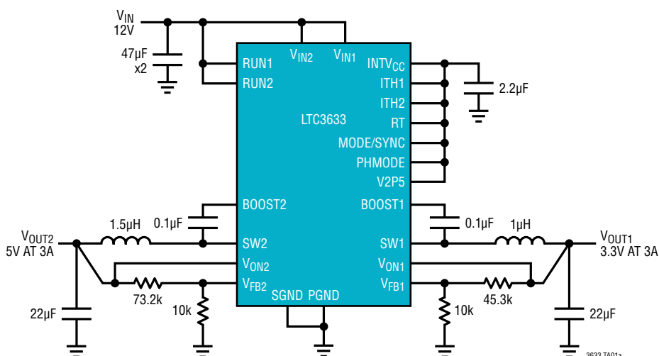
Comparable Switching Regulator Solution (LTC3633 Demo Circuit 1347A Dual 3A Output)
