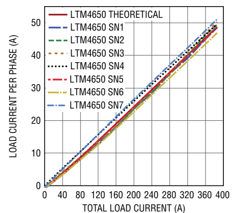
DC2481A-B + DC2455A-C. Current Sharing.
