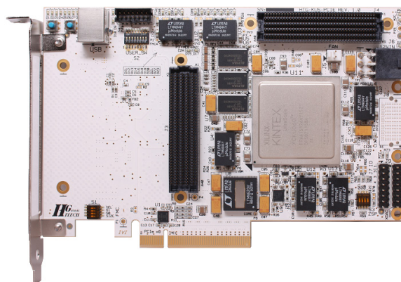
Xilinx Kintex Ultrascale PCI Express Platform (by HiTech Global)
