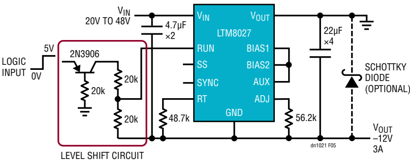
LTM8027 Can Be Easily Configured to Generate Negative Output Voltages. Run Voltage Must Be Level-Shifted.
