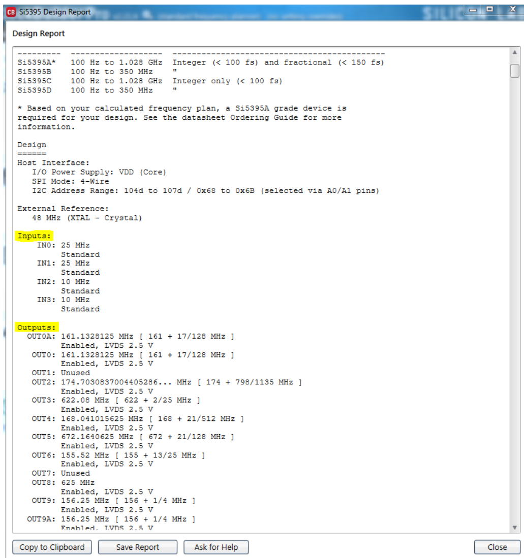
Figure 10.12. Design Report Window
