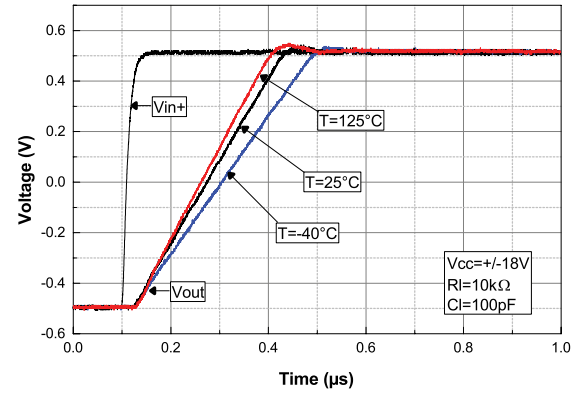
Figure 20. Positive slew rate at V_{CC} = 36\text{ V}
