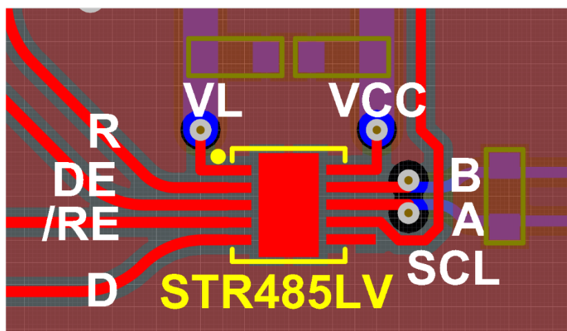
Figure 3. Example of implementation in a PCB
