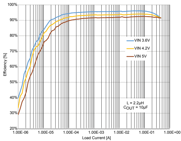
Figure 6. Efficiency vs load, V_{OUT} = 3.3\text{ V}
