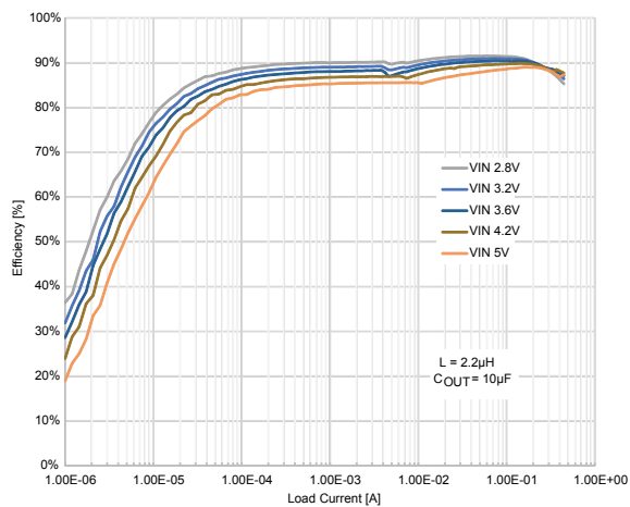
Figure 4. Efficiency vs load, V_{OUT} = 1.8\text{ V}
