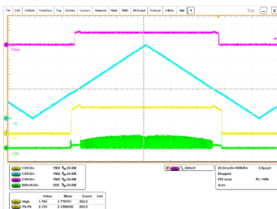
Figure 8. 100% mode, V_{OUT} = 1.8\text{ V}
