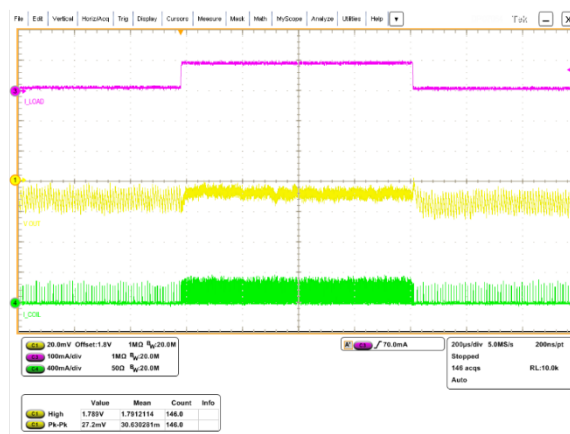
Figure 22. Load transient, V_{IN}=3.6\text{ V} , V_{OUT}=1.8\text{ V} , I_{OUT}=0 to 100\text{ mA}
