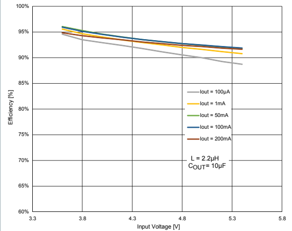
Figure 7. Efficiency vs V_{IN} , V_{OUT} = 3.3\text{ V}
