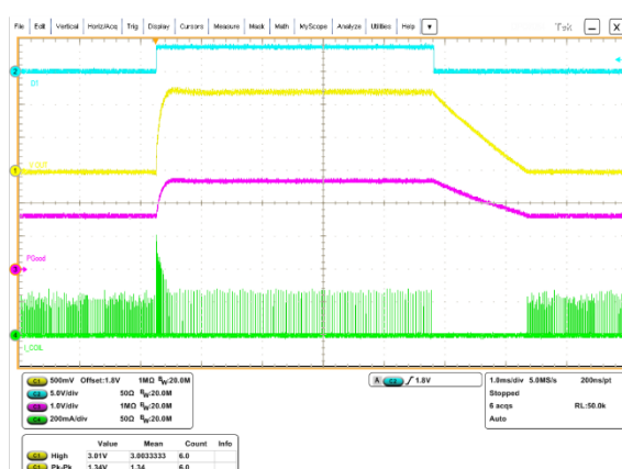
Figure 10. V_{OUT} change, 1.8 V to 3.3 V to 1.8 V, I_{OUT}=5 mA
