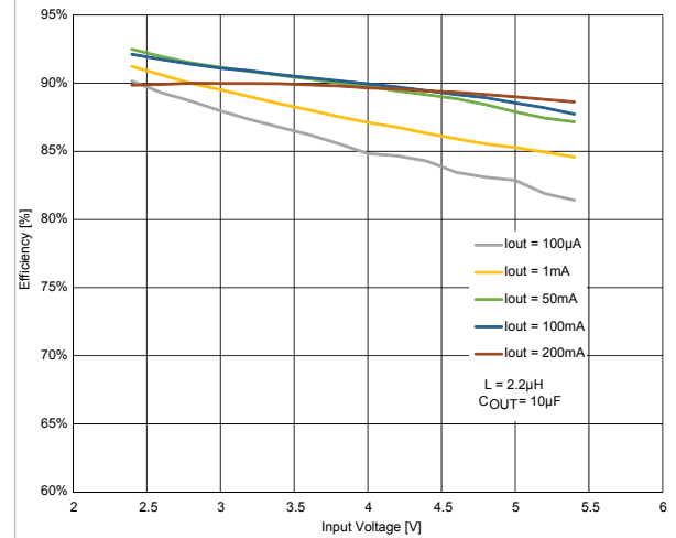
Figure 5. Efficiency vs V_{IN} , V_{OUT} = 1.8\text{ V}
