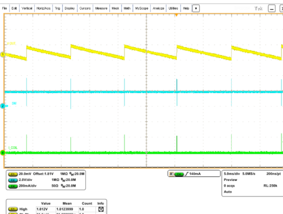
Figure 12. Output ripple, V_{IN}=3.6\text{ V} , V_{OUT}=1.8\text{ V} , I_{OUT}=10\text{ mA}
