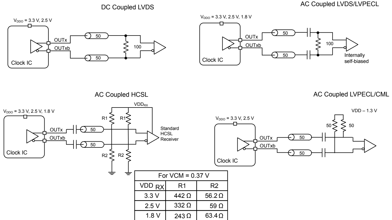
Figure 6.2. Supported Differential Output Terminations
