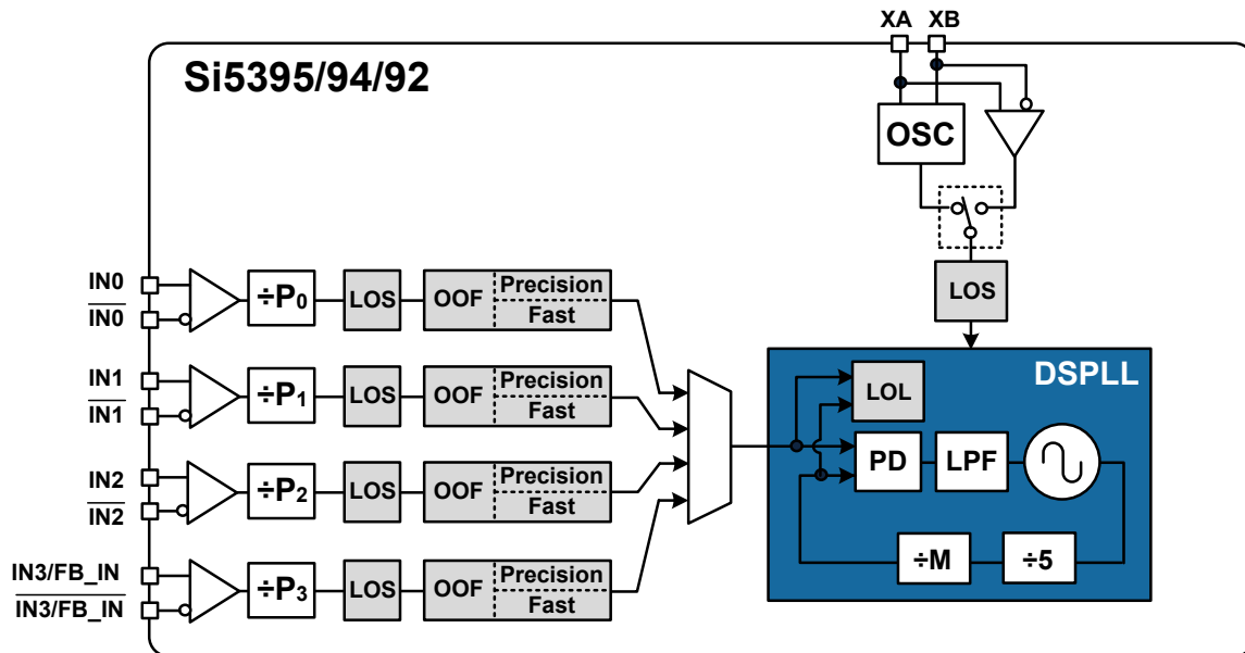
Figure 5.5. Fault Monitors
