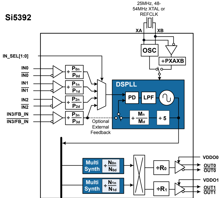
Figure 3.1. Si5392 DSPLL and MultiSynth System Flow Diagram
