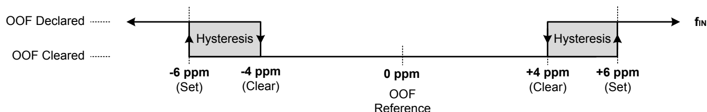
Figure 5.9. Example of Precise OOF Monitor Assertion and De-assertion Triggers
