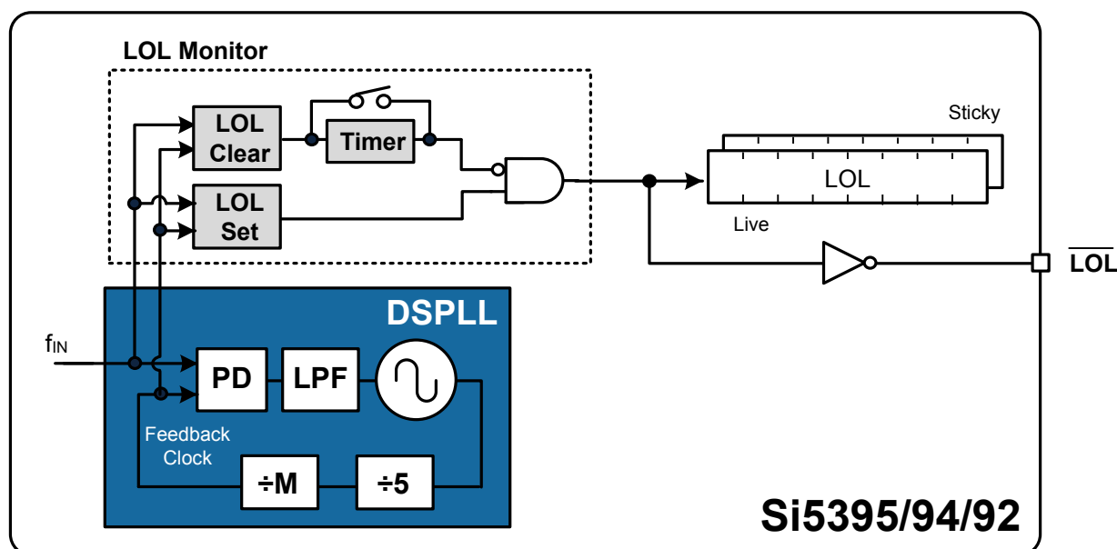
Figure 5.10. LOL Status Indicators
