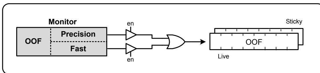
Figure 5.8. OOF Status Indicator
