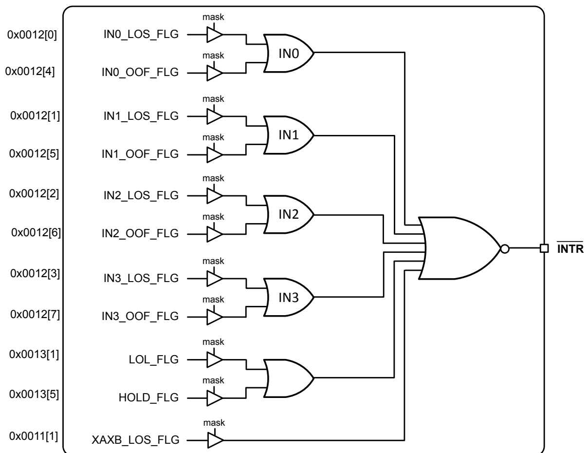
Figure 5.12. Interrupt Triggers and Masks
