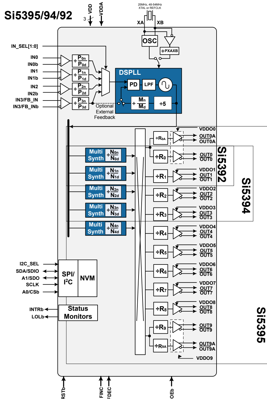
Figure 2.1. Block Diagram Si5395/94/92
