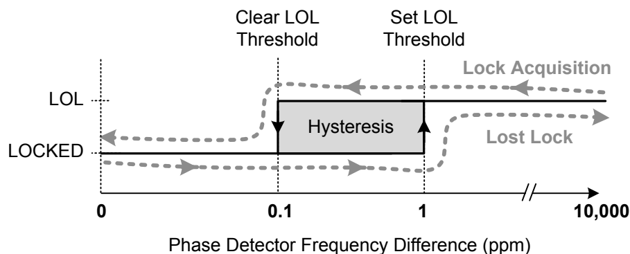
Figure 5.11. LOL Set and Clear Thresholds
