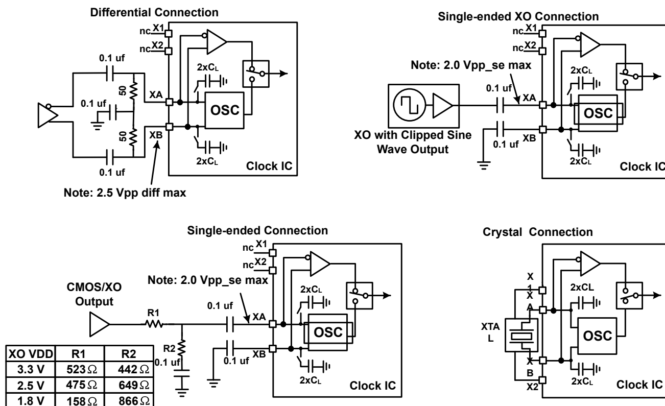
Figure 11.1. XAXB Crystal Resonator and External Reference Clock Connection Options
