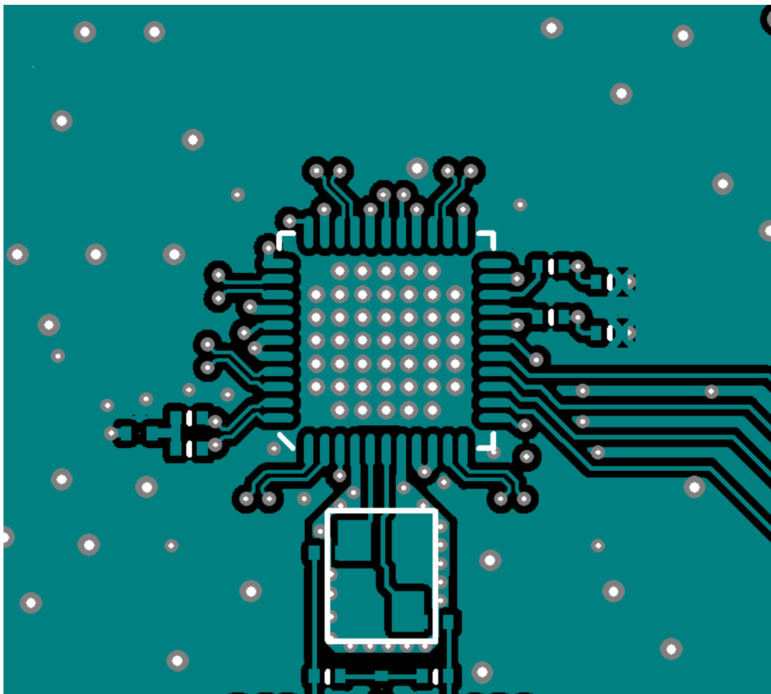
Figure 12.9. Device Layer (Layer 1)
