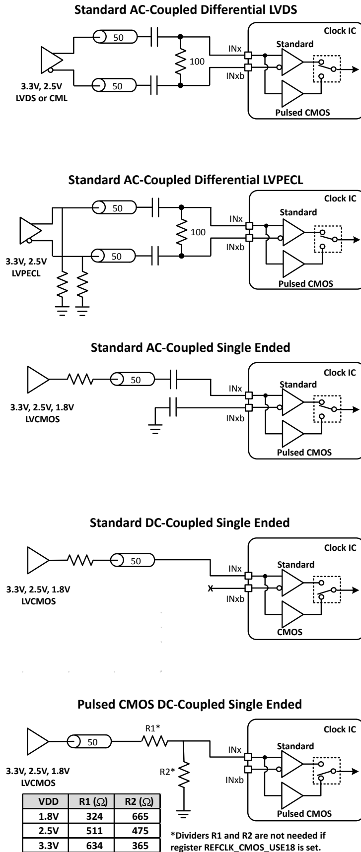
Figure 5.2. Input Termination for Pulsed CMOS Inputs
