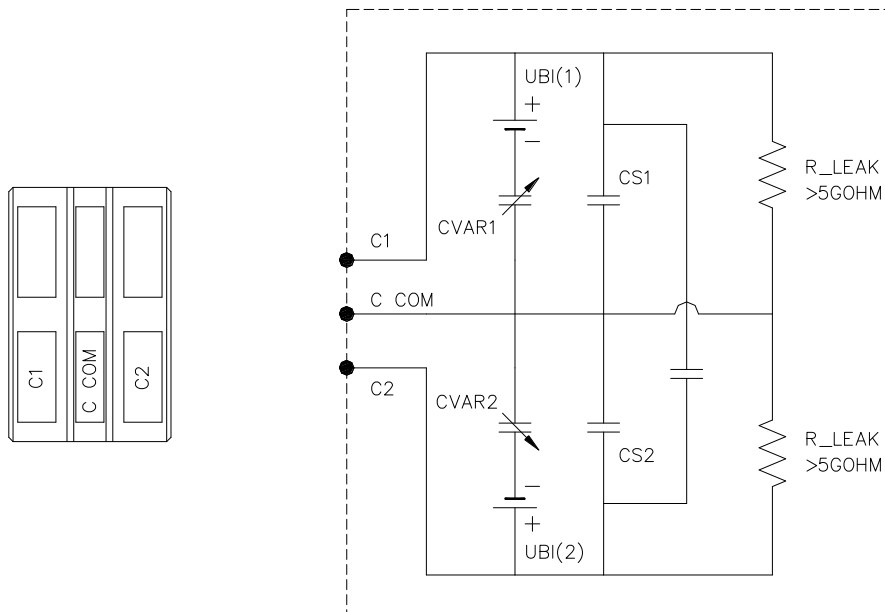
SCG10X Series sensing element equivalent circuit and connections
