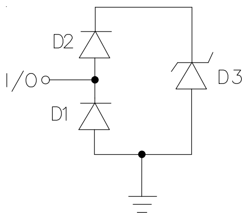
RClamp0522P Spice Model
