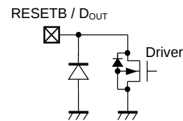
Equivalent Circuit for RESETB Pin (R5115Sxx1x)/ Equivalent Circuit for DOUT Pin (R5115Sxx2C)
