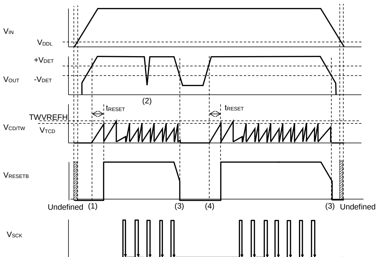
R5115Sxx1A/ R5115Sxx1B VD Timing Chart
