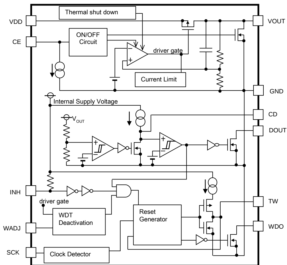
R5115Sxx2C Block Diagram
