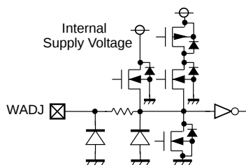
Equivalent Circuit for WADJ Pin (R5115Sxx2C)
