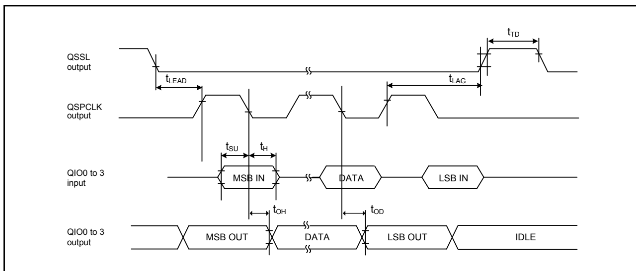
Figure 2.65 Transfer/receive timing
