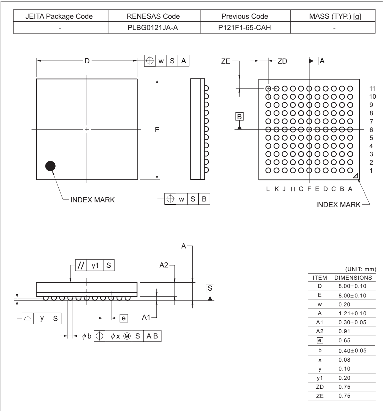
Figure 1.3 BGA 121-pin
