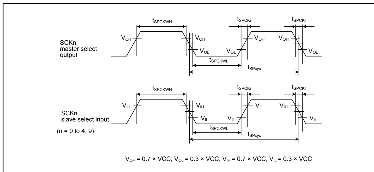
Figure 2.51 SCI simple SPI mode clock timing
