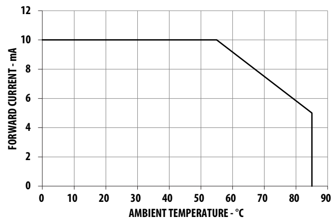
Figure 7 Derating Curve
