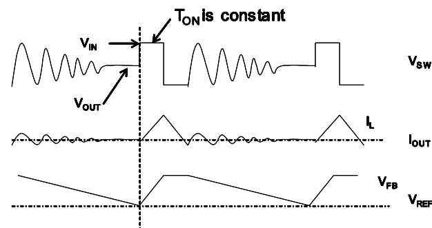
Figure 3: Light-Load Operation
