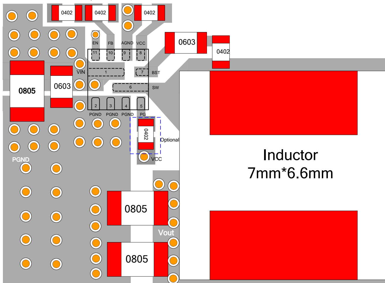
Figure 10: Recommended Layout
