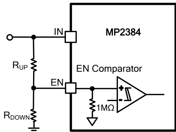
Figure 7: Adjustable UVLO
