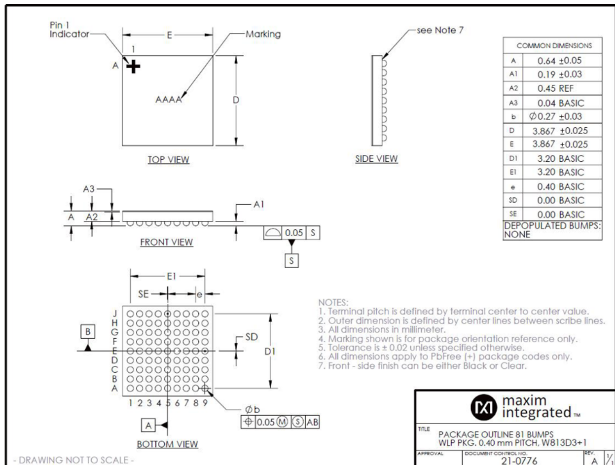
Figure 2. Package outline drawing of a 0.4mm pitch WLP.
