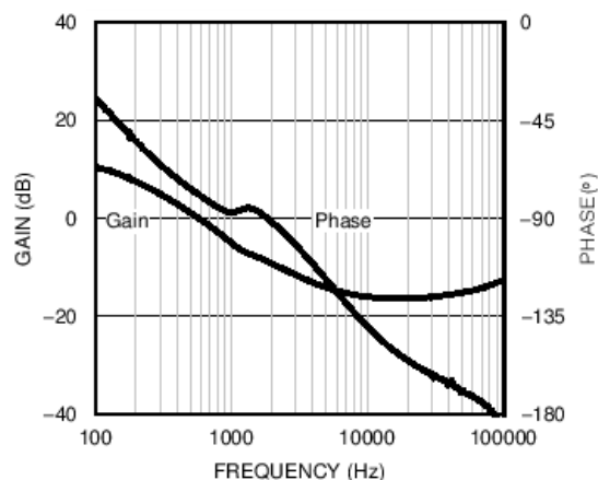
Figure 22. Modulator Gain and Phase - Buck-Boost Mode
