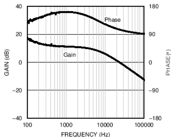
Figure 23. Error Amplifier Gain and Phase - Buck Mode
