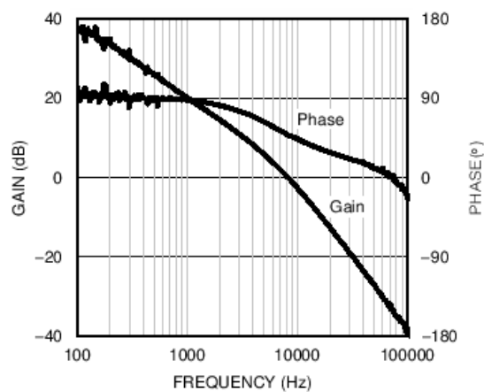
Figure 25. Overall Loop Gain and Phase - Buck Mode
