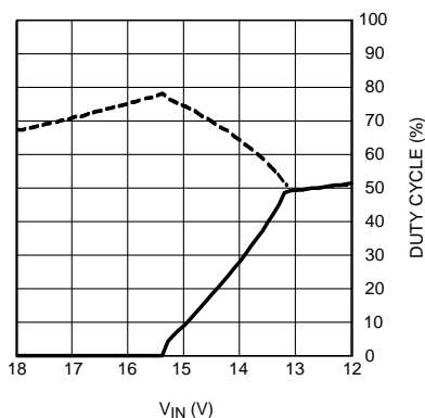
Figure 12. Mode Dependence on Duty Cycle (V OUT = 12 V)
