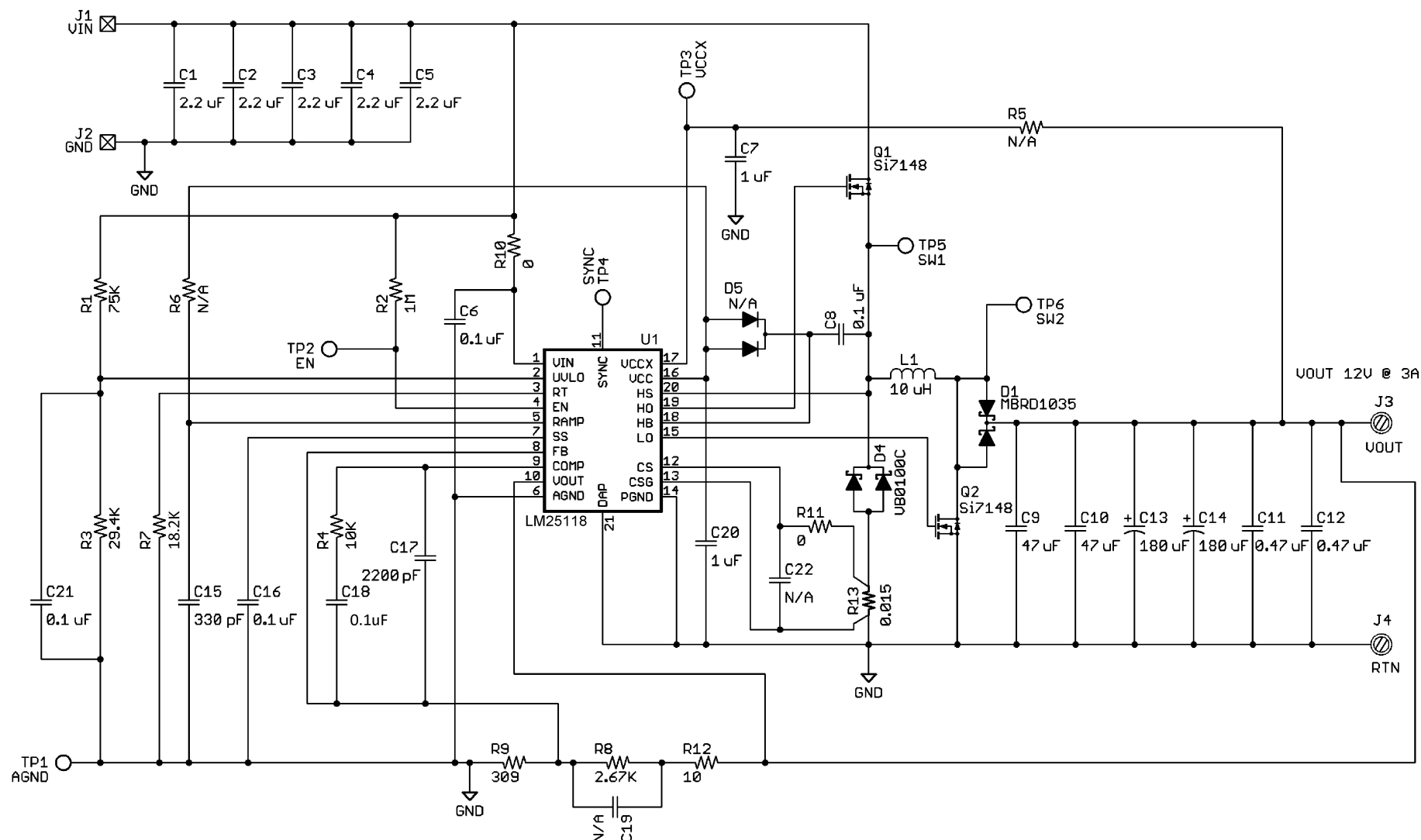
Figure 29. 12 V, 3 A Typical Application Schematic
