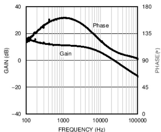
Figure 24. Error Amplifier Gain and Phase - Buck-Boost Mode
