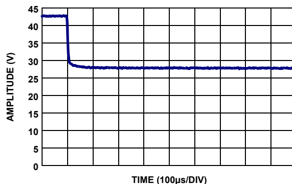
FIGURE 61. CFET FALL
