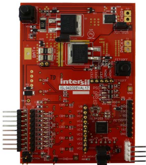
FIGURE 2. ISL94202EVKIT1Z TOP OF BOARD
