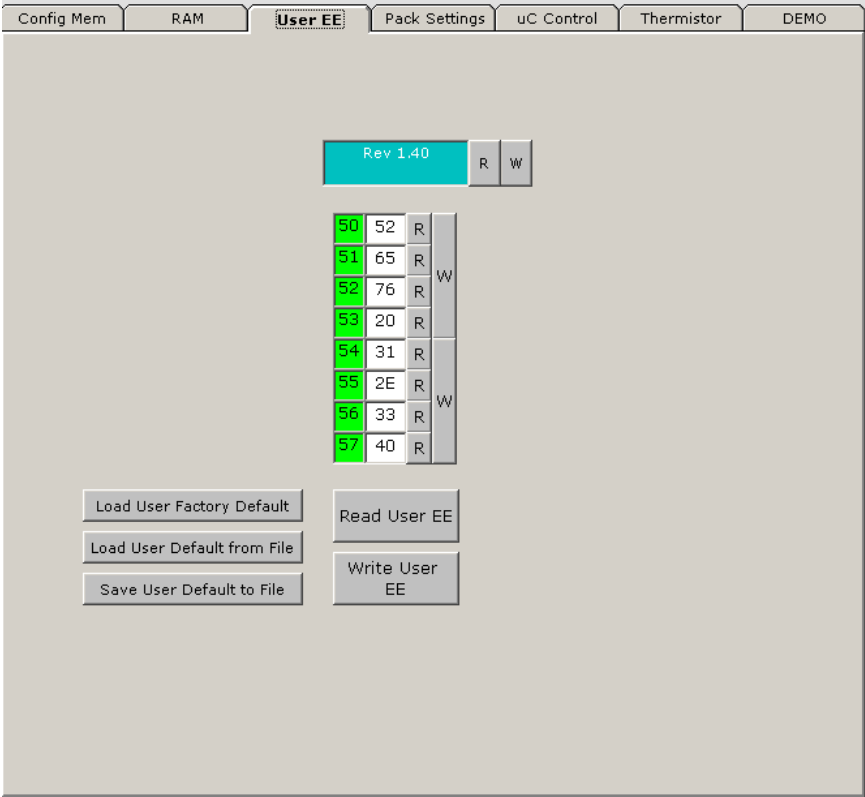
FIGURE 30. ISL94202 GUI - USER EEPROM TAB
