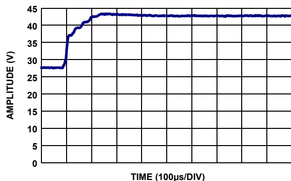
FIGURE 60. CFET RISE
