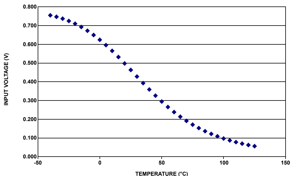
FIGURE 12. VOLTAGE TO TEMPERATURE CONVERSION
