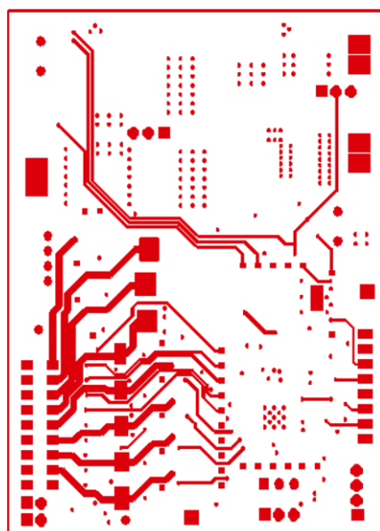
FIGURE 54. MIDDLE LAYER 2
