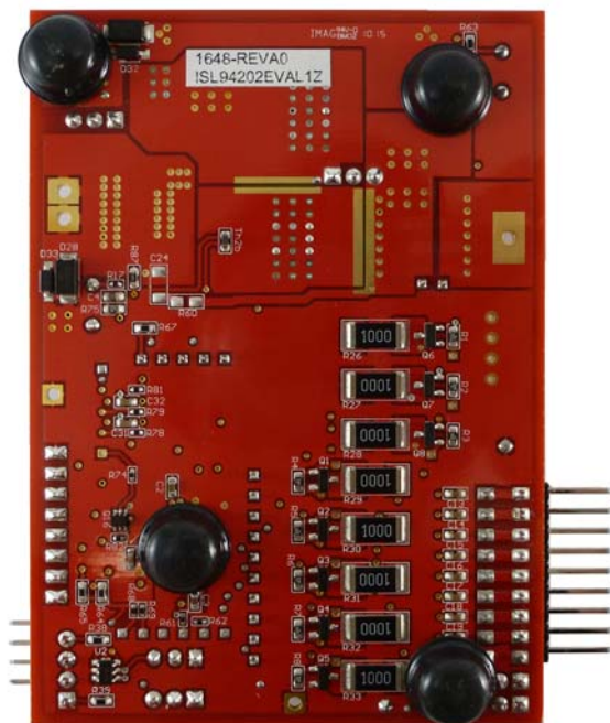
FIGURE 3. ISL94202EVKIT1Z BOTTOM OF BOARD
