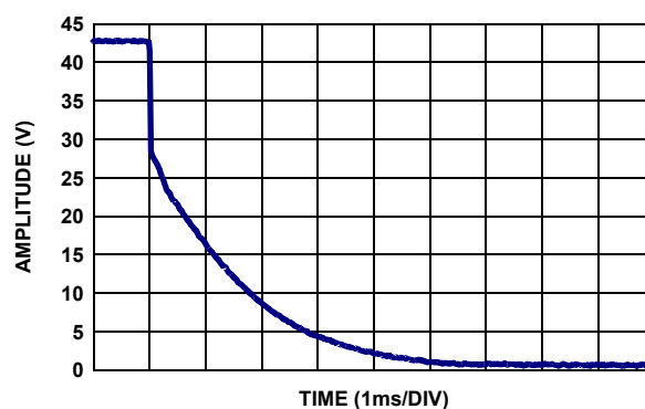
FIGURE 59. DFET FALL
