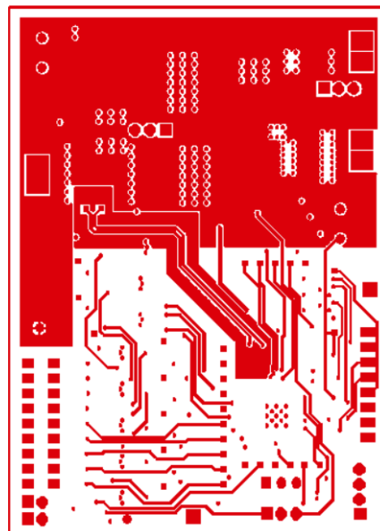
FIGURE 53. MIDDLE LAYER 1
