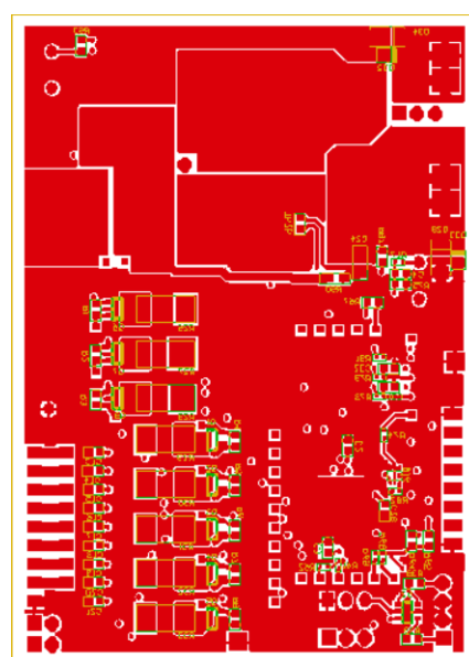
FIGURE 55. BOTTOM LAYER
