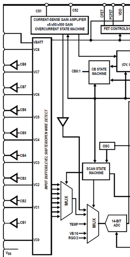
FIGURE 24. ANALOG MUX
