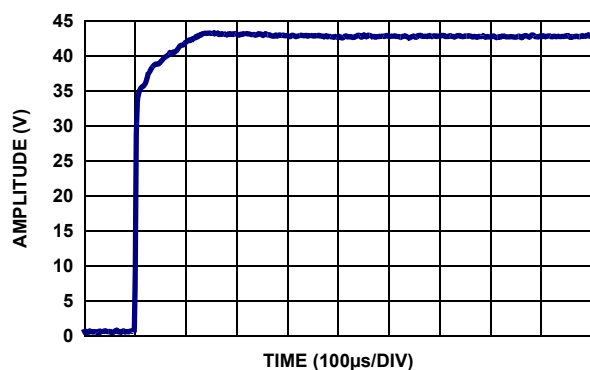
FIGURE 58. DFET RISE
