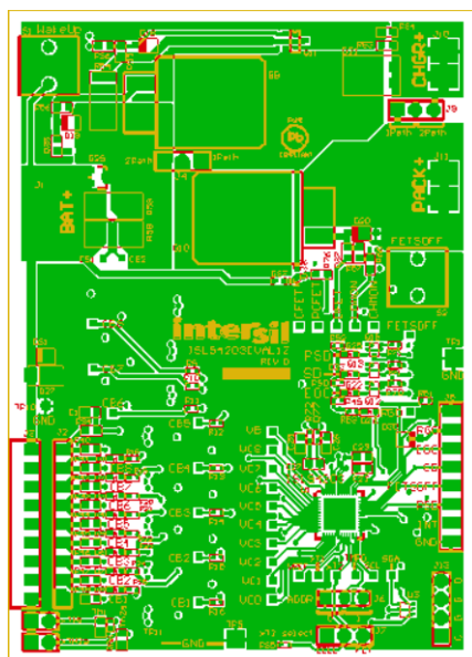
FIGURE 52. TOP LAYER
