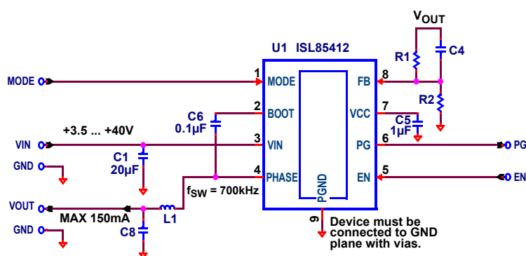
FIGURE 1. TYPICAL APPLICATION
