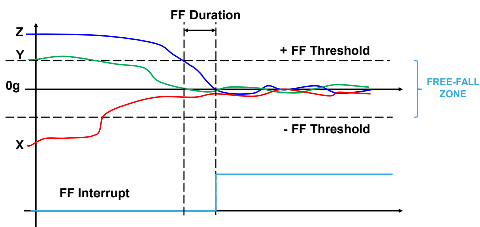
Figure 13. Free-fall interrupt
