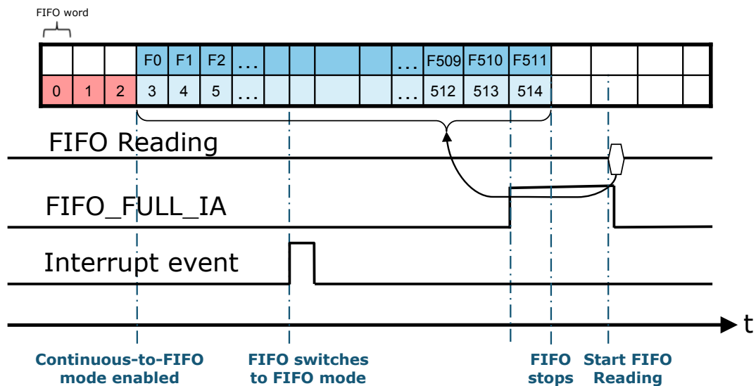
Figure 30. Continuous-to-FIFO mode
