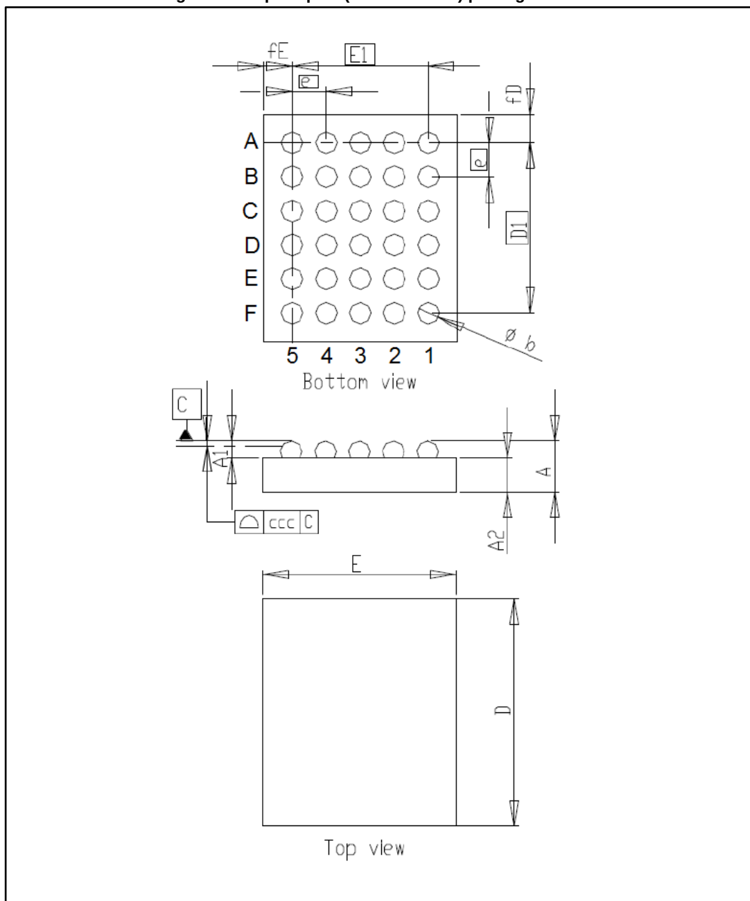
Figure 23: Flip Chip 30 (2.59x2.25 mm) package outline
