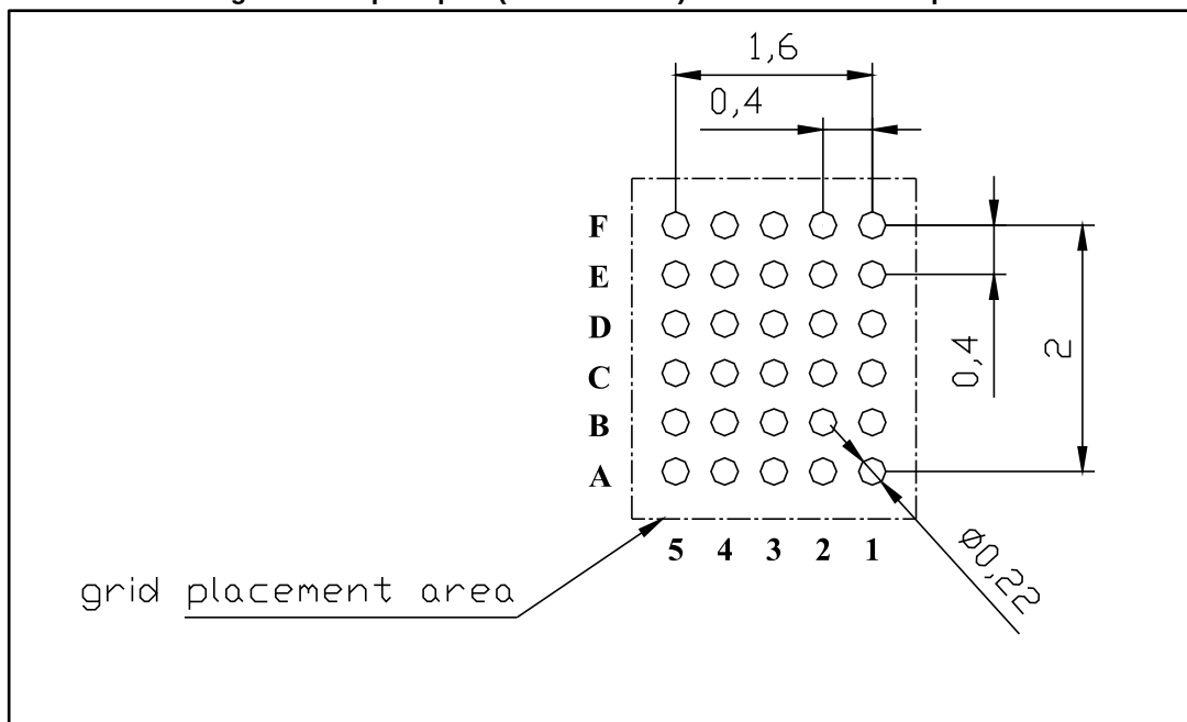
Figure 24: Flip Chip 30 (2.59x2.25 mm) recommended footprint
