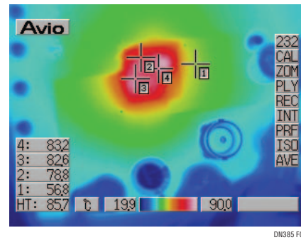
Figure 4. The LTM4600 Exhibits Impressive Thermal Performance, Even Without Air Flow and Heat Sink (24V to 3.3V at 10A, Top View). For a Color Representation, Download the File at www.linear.com
