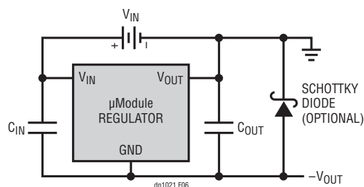
Figure 6. Step-Down \mu Module Regulator with Schottky Diode Protection for Negative Output
