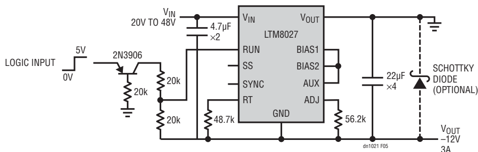
Figure 5. LTM8027 with Run Level-Shift Circuitry for -12V Output
