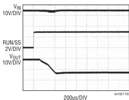
Figure 3. LTM8025 Start-Up Waveforms for -12V Output
