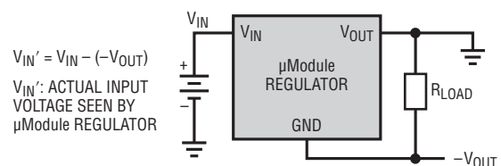
(b) Buck \mu Module Regulator Configured for Negative Output Voltages
