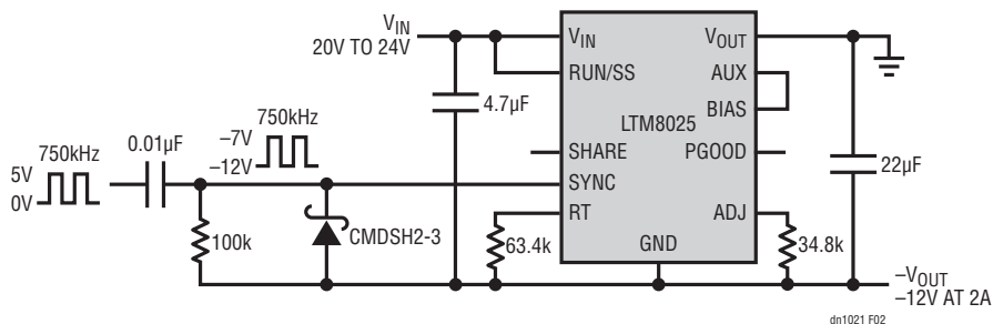
Figure 2. LTM8025 Schematic for -12V Output
