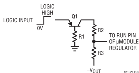
Figure 4. Run Level-Shift Circuit for Negative Output Configuration
