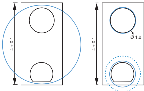
Fig. 10 - Light Holes Diagrams
