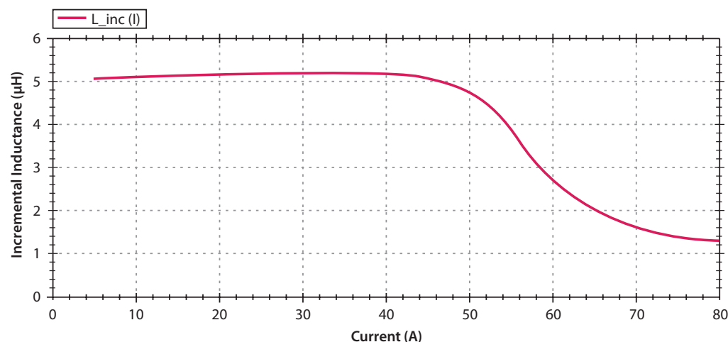
Figure 3. | The Model PQ series products offer a high operating temperature specified at 150 °C
