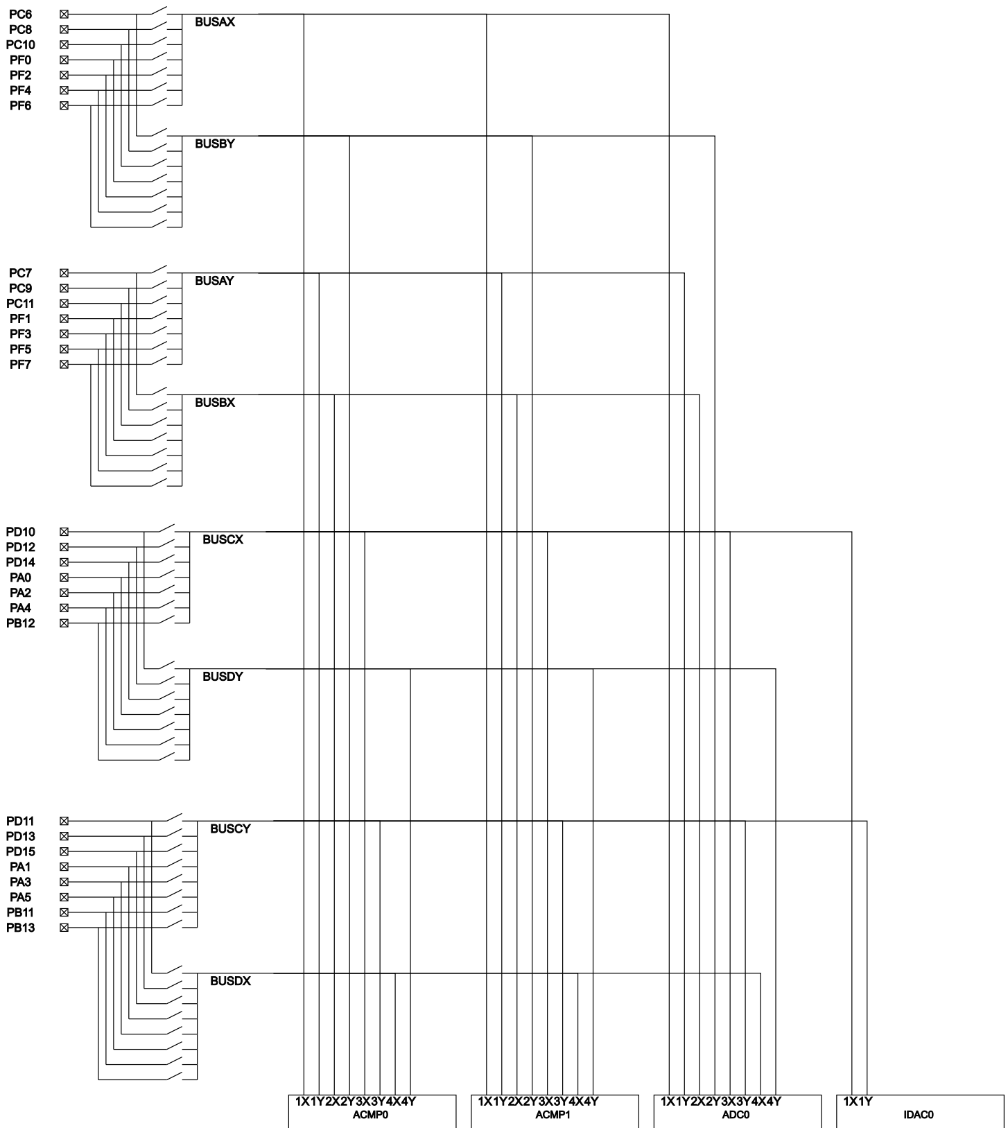
Figure 7.2. BGM121/BGM123 APORT
