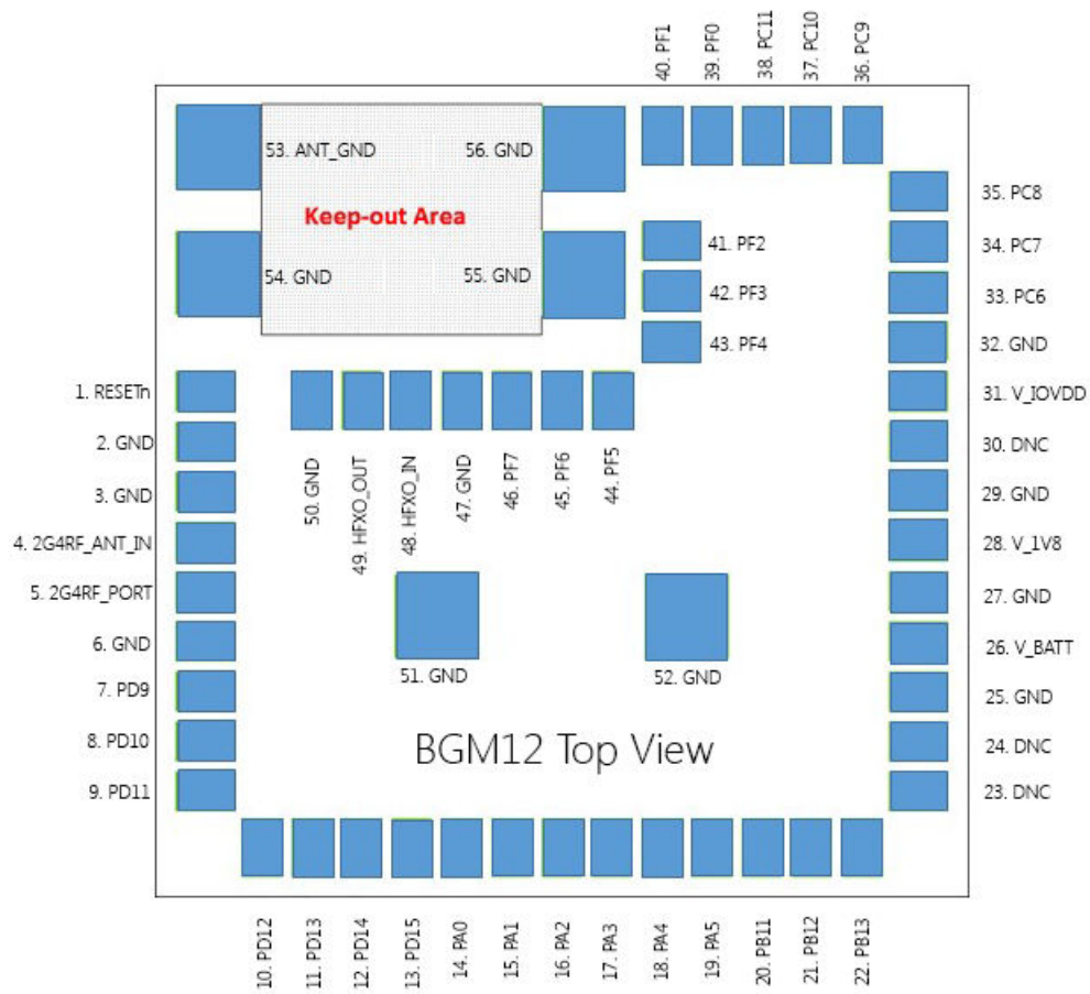
Figure 7.1. BGM121/BGM123 Pinout
