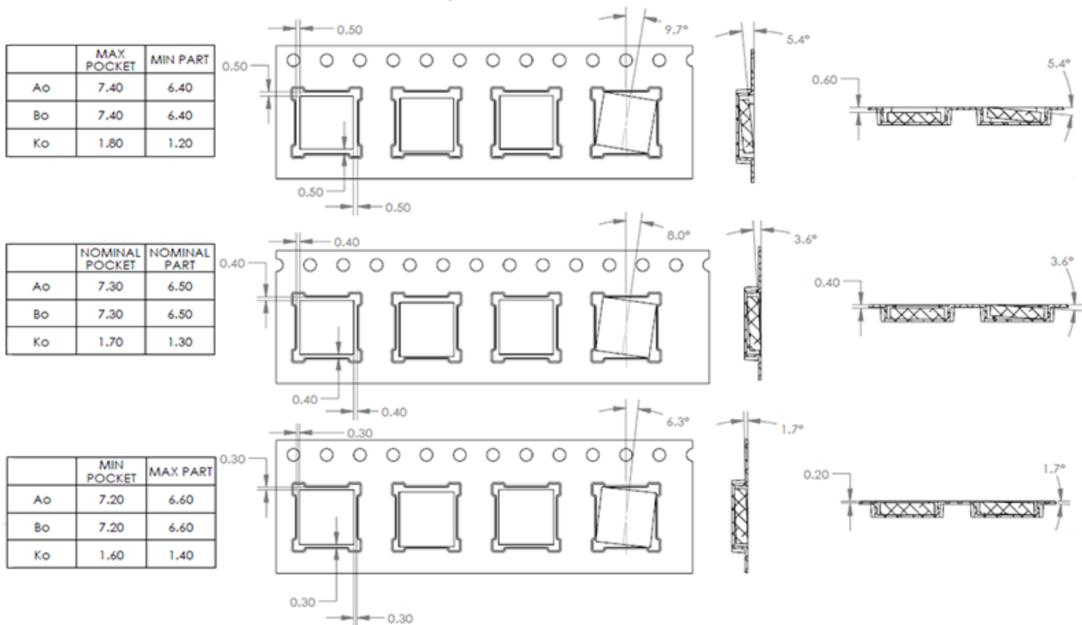
Figure 9.3. Tape information
