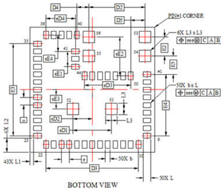
Figure 8.1. BGM121/BGM123 Package Dimensions
