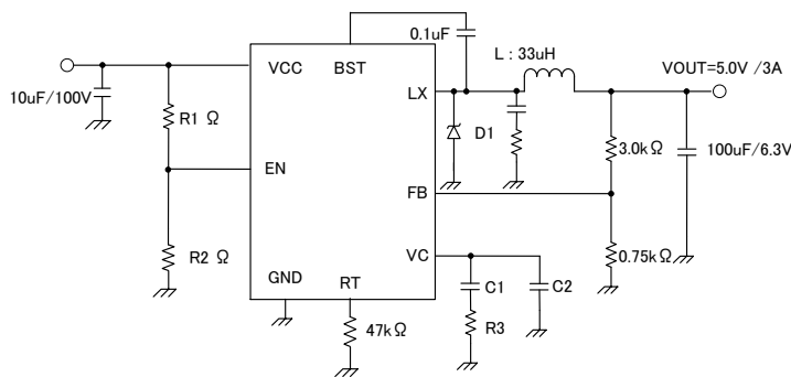
Fig.34 Feedback voltage resistance setting method
