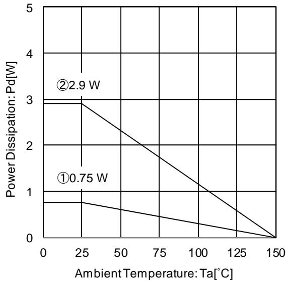
Figure 44. Package Data (HTSOP-J8)
