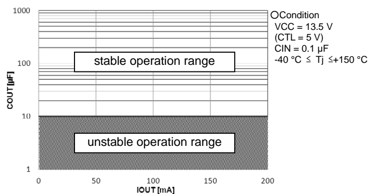
Figure 42. COUT vs. IOUT
