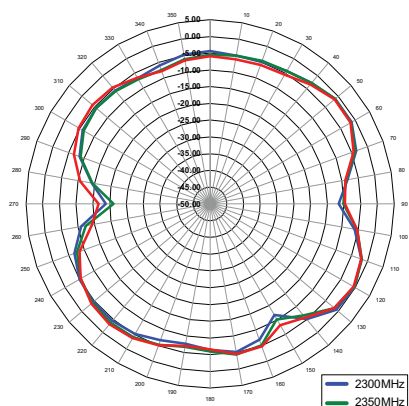
XY-Plane Gain
