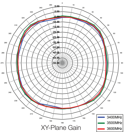
XY-Plane Gain
