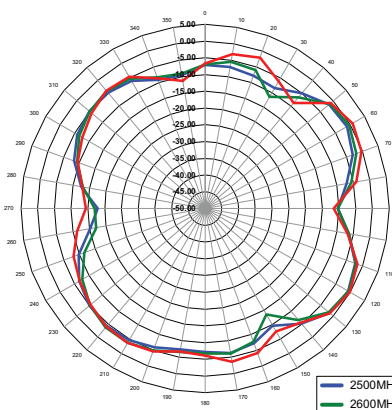
XY-Plane Gain
