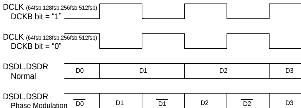
Figure 51. DSD mode Timing
