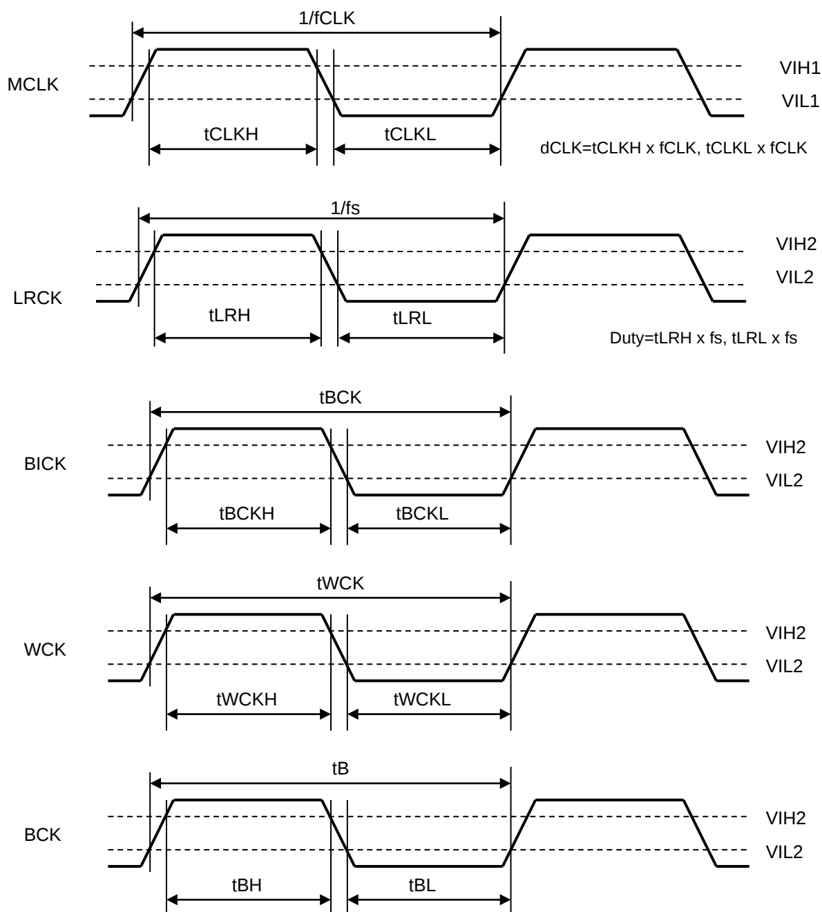
Figure 13. Clock Timing
