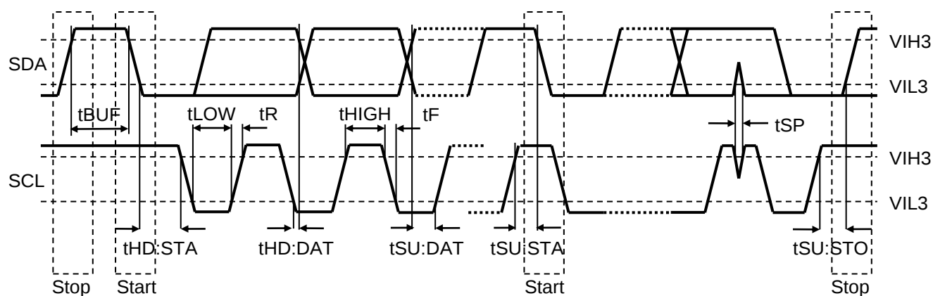
Figure 20. I 2 C-bus Timing
