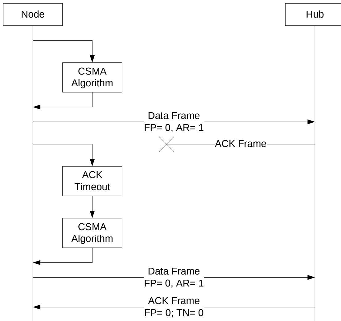
Figure 17 • Failed ACK Response, Hub to Node
