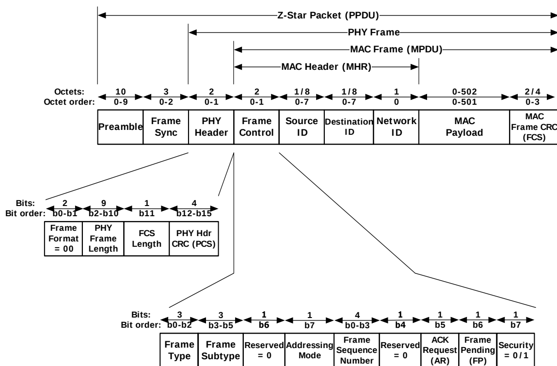
Figure 2 • Z-Star Normal Frame Format
