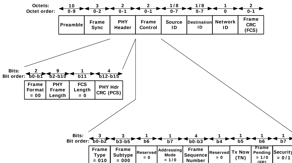
Figure 4 • Z-Star Acknowledgment Frame Format
