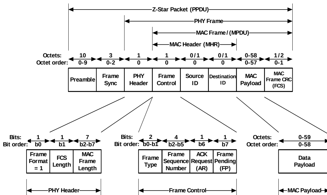
Figure 7 • Short Frame Format
