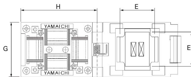
Outline Clamshell Socket Dimensions
