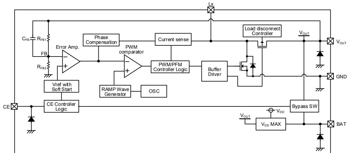
XC9141B/XC9142B type
