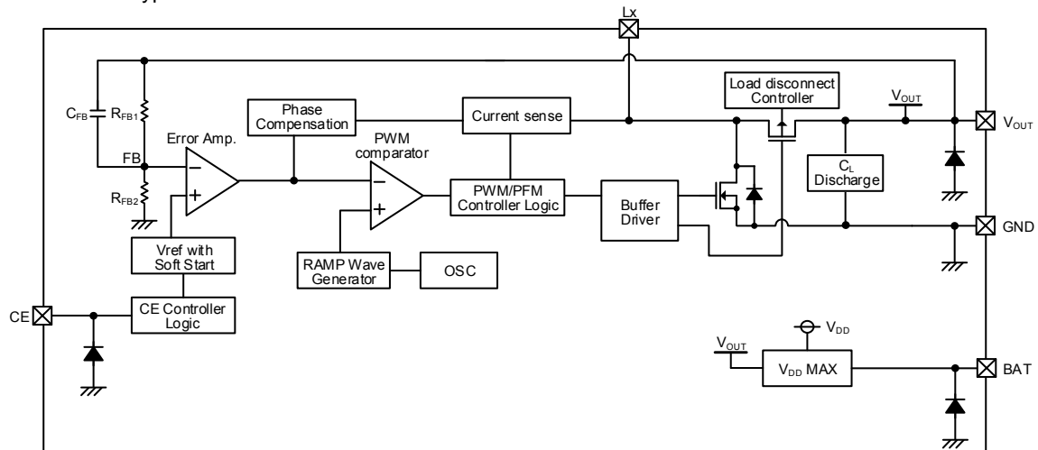
XC9141A/XC9142A type
