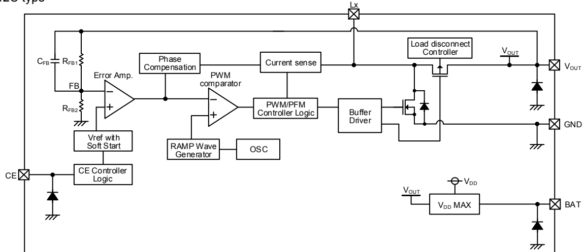
XC9142C type
