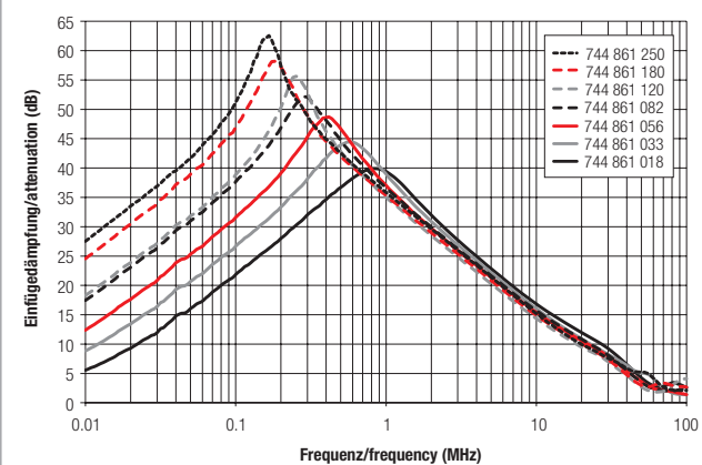
Insertion loss common mode
