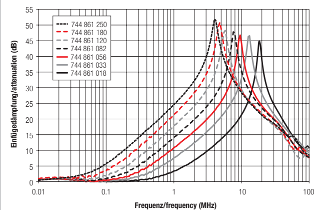
Insertion loss differential mode
