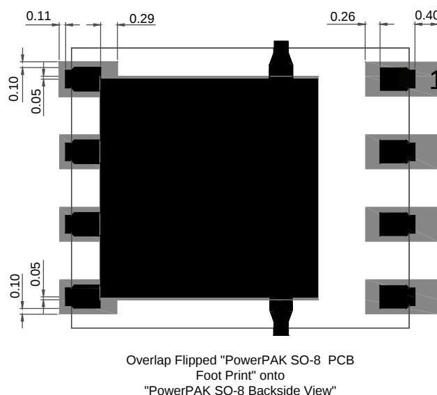
Fig. 6 - Single Channel PowerPAK SO-8 on its PAD Layout
