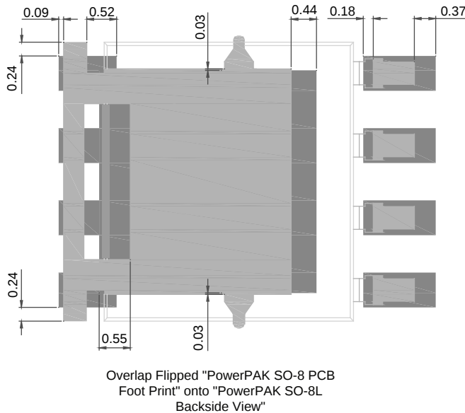
Fig. 7 - Single Channel PowerPAK SO-8L on Single Channel PowerPAK SO-8 PAD Layout
