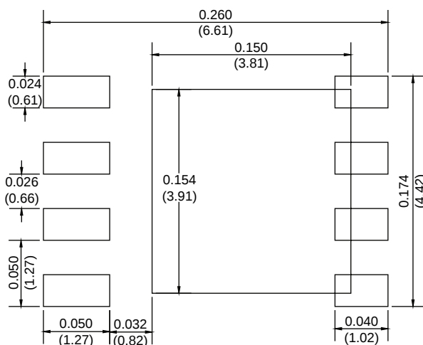
Fig. 5 - Recommended Minimum PADs for PowerPAK SO-8 Single Dimensions in Inches/(mm)
