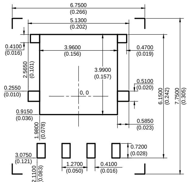
Fig. 8 - Recommended PAD for Single Channel Power PAK SO-8L Dimensions in mm (inches) Keep-out 6.75 (0.266) x 7.75 (0.305)
