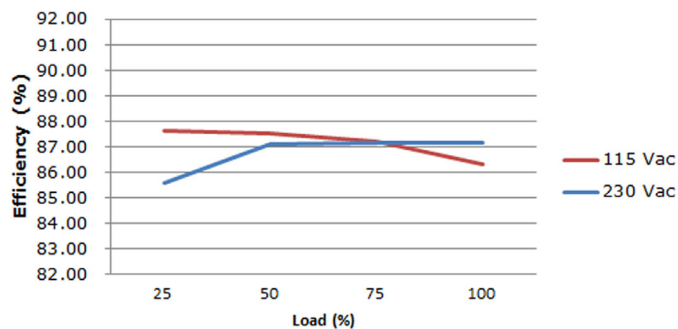
VOF-50B-12 Efficiency vs. Output Load (Natural Convection)
