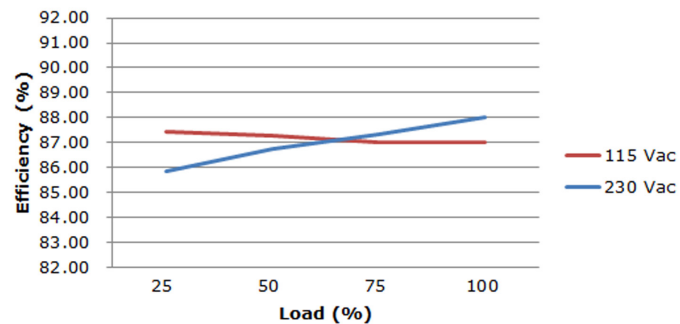
VOF-50B-15 Efficiency vs. Output Load (Natural Convection)
