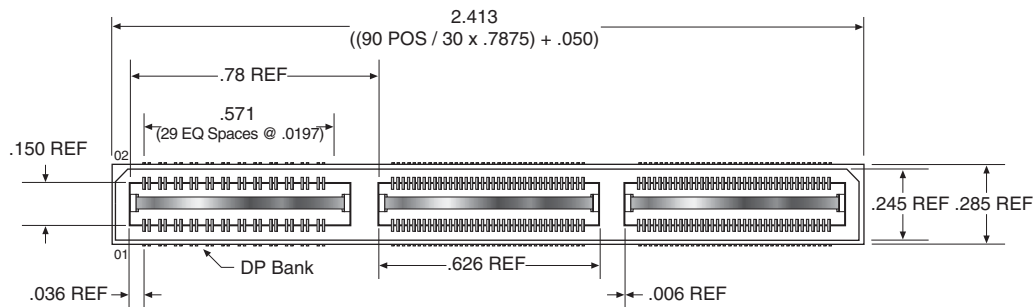
Figure 2–7. Samtec Header Connector
