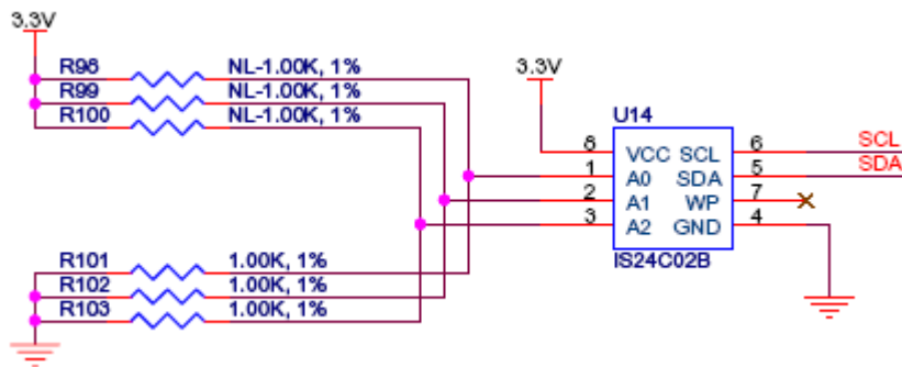
Figure 2–8. I2C Serial EEPROM Schematic
