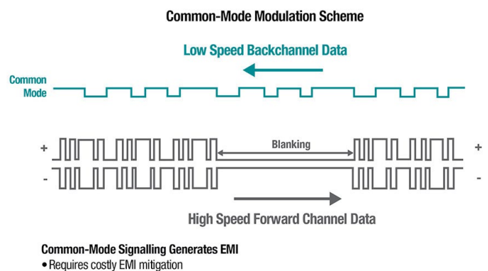
Figure 2 Control channel implemented using common-mode modulation of video data
