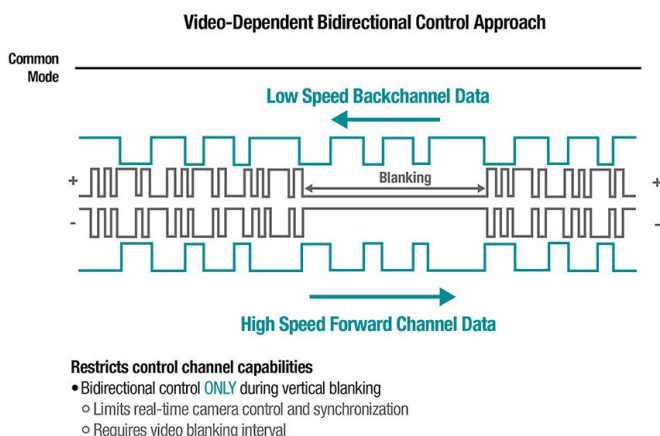
Figure 1. Control Channel implemented during video banking
