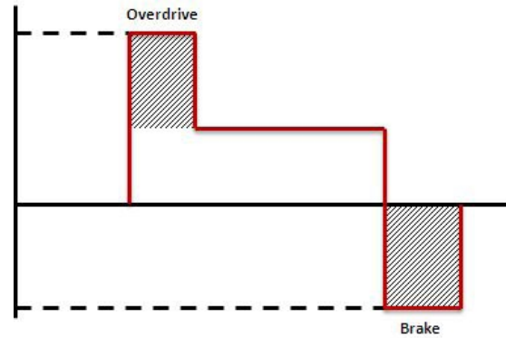
Figure 4: ERM Overdrive and Braking Drive Waveform
