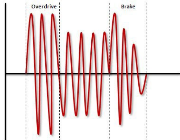
Figure 5: LRA Overdrive and Braking Drive Waveform
