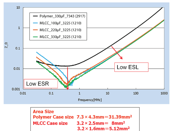
Figure 1. MLCCs of 100 \mu F, 220 \mu F and 330 \mu F compared with a polymer capacitor
