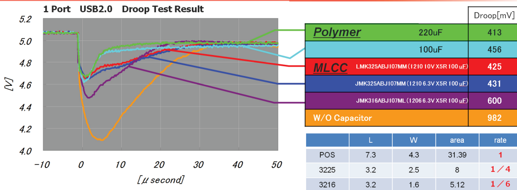
Figure 2. Droop test performance of MLCCs similar to comparable electrolytics
