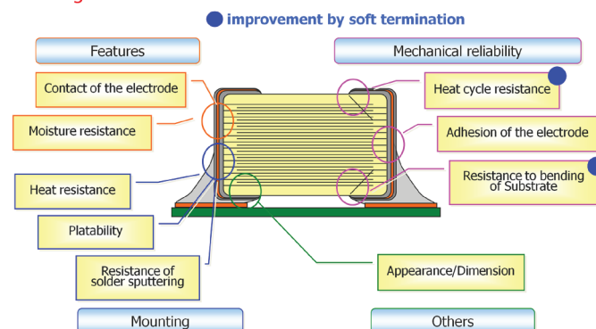
Figure 14. MLCCs' soft-termination provides heat-cycle resistance and resistance to substrate bending.
