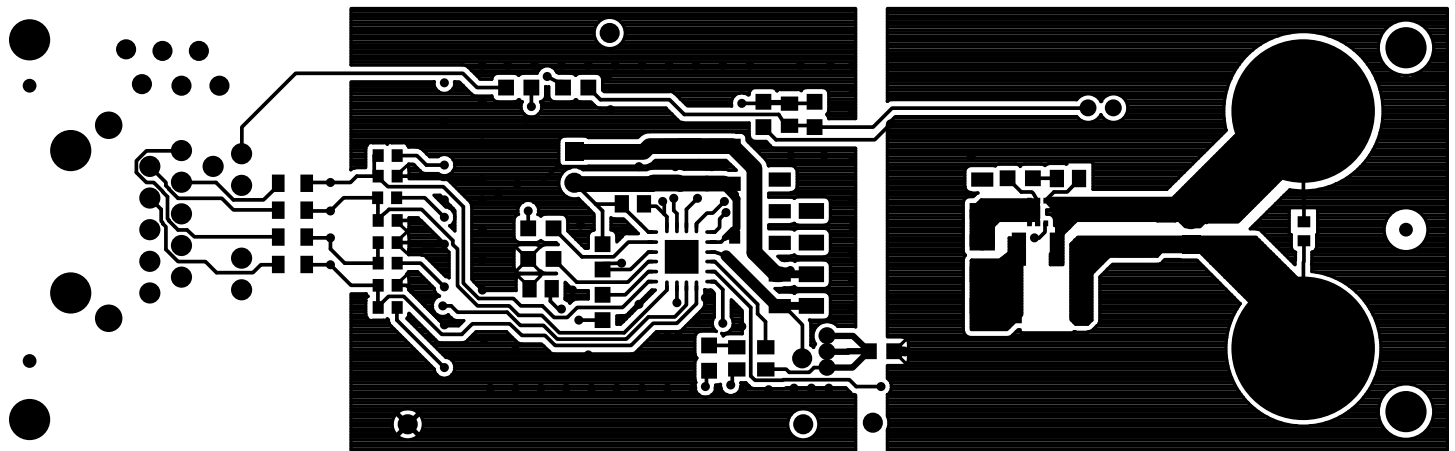
PRIMARY SIDE
