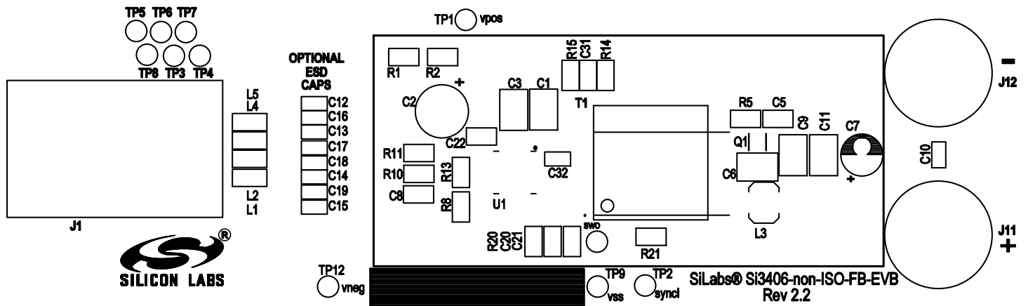
PRIMARY SILKSCREEN
