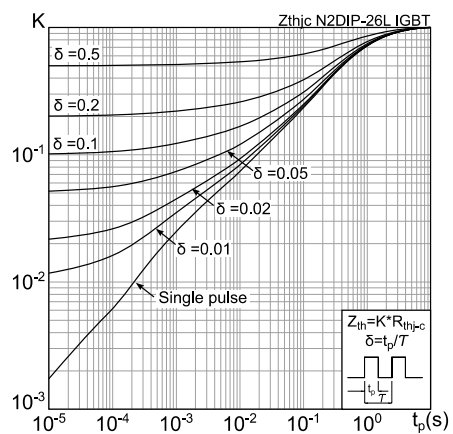
Figure 16: Thermal impedance for IGBT
