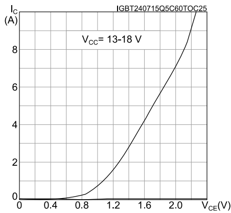
Figure 11: Output characteristics
