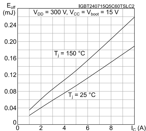
Figure 15: E_{off} switching energy vs collector current
