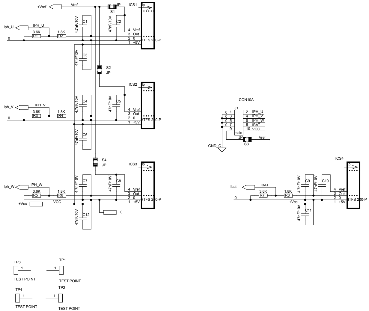
Figure 1: STEVAL-CTM008V1 current sensing board schematic
