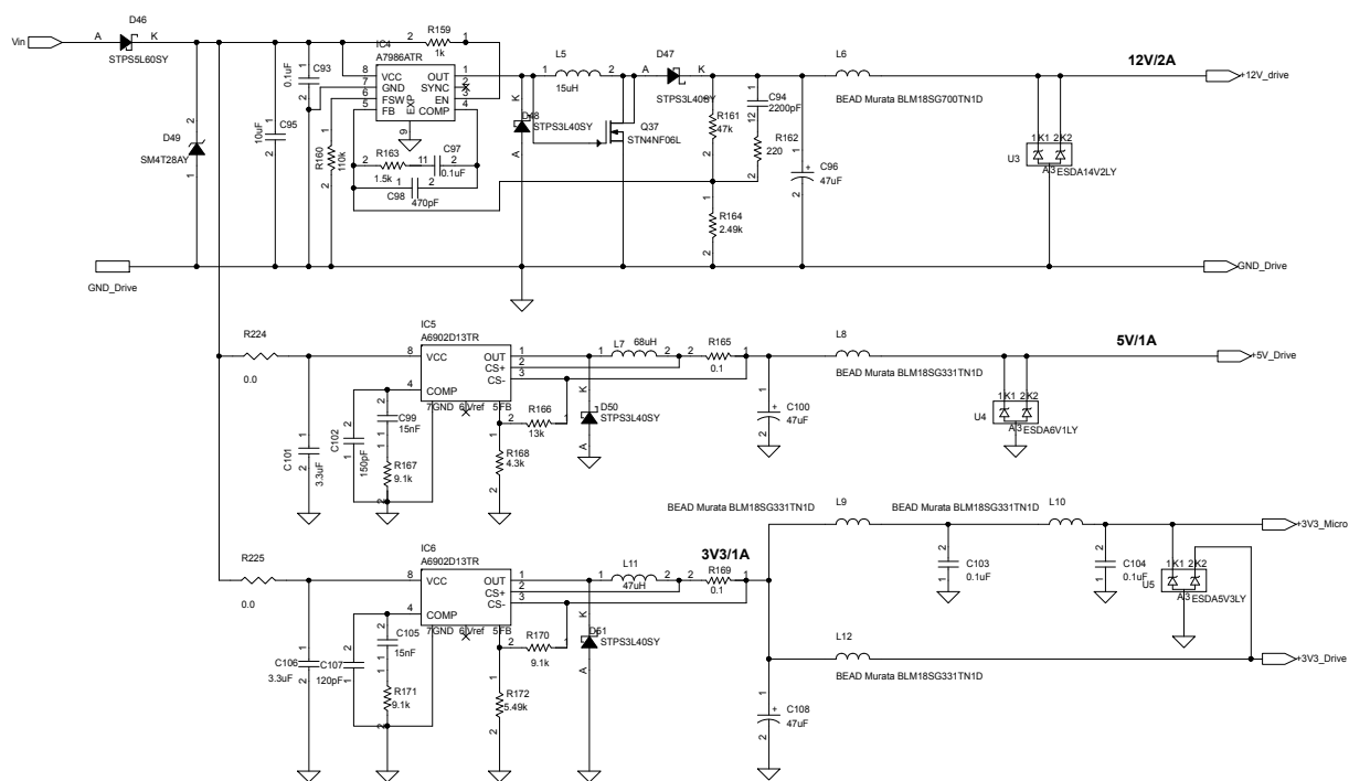
Figure 5: STEVAL-CTM006V1 driver board schematic - power supply
