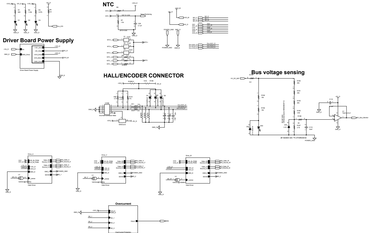
Figure 2: STEVAL-CTM006V1 driver board schematic - sensing
