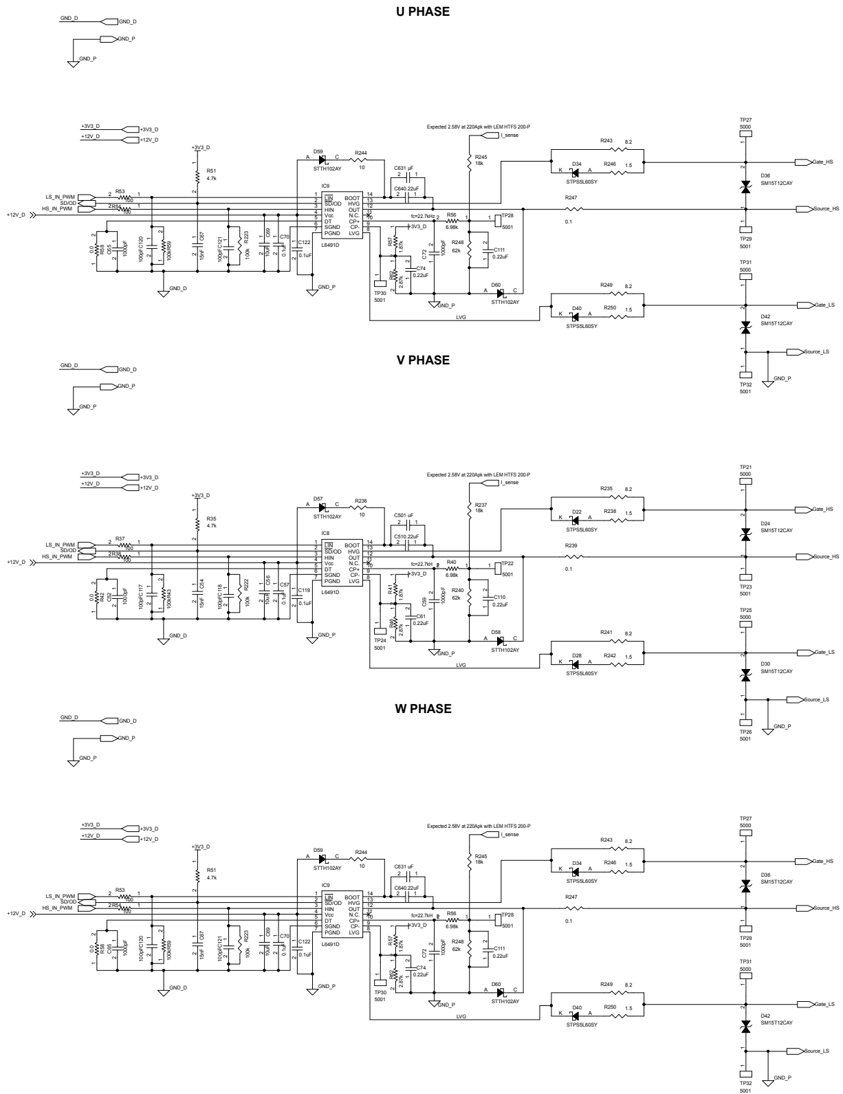
Figure 3: STEVAL-CTM006V1 driver board schematic - gate drivers
