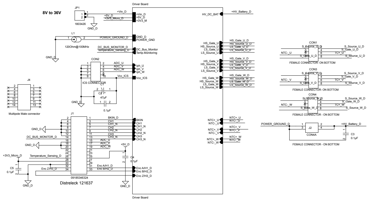
Figure 2: STEVAL-CTM006V1 driver board schematic - sensing
