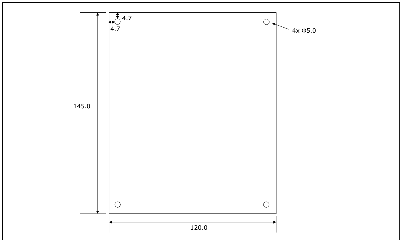
Figure 2.2 Overlay Dimensions
