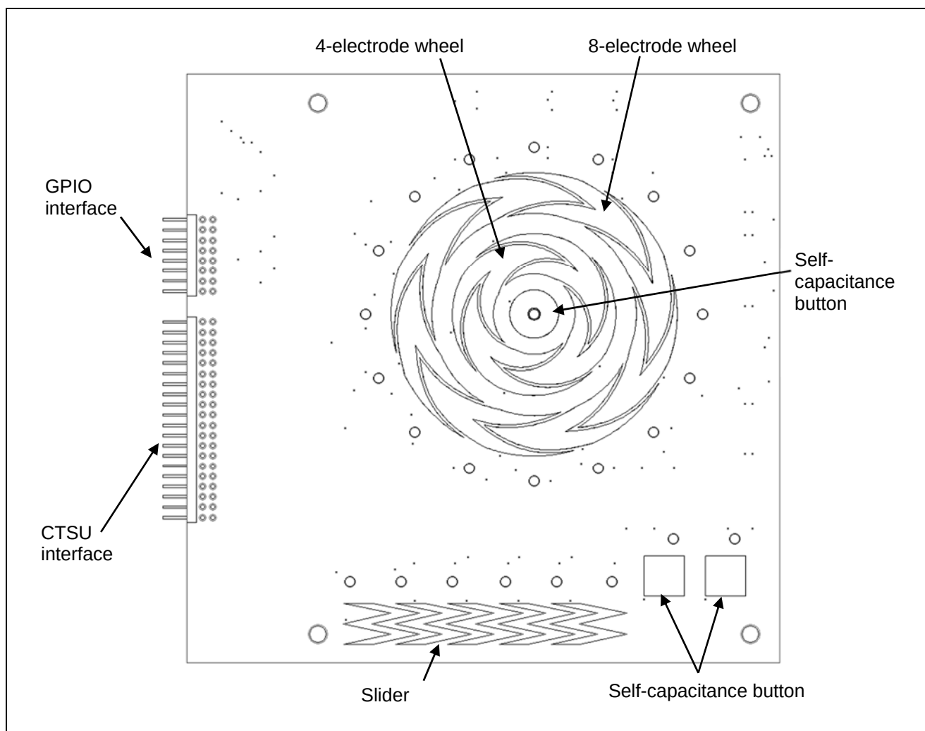
Figure 2.1 Component Layout
