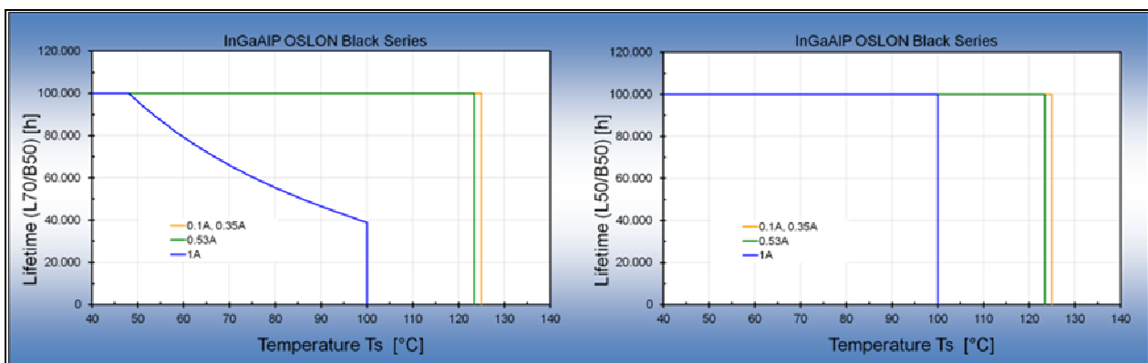
Figure 7: Lifetime (*) of the OSLO Black Series with ThinFilm technology with respect to T_s
