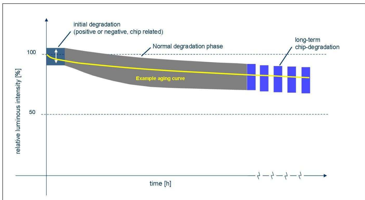
Figure 4: Degradation characteristics of the OSRON Black Series group
