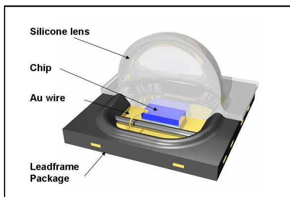
Figure 2: Construction of the OSOLON Black Series
