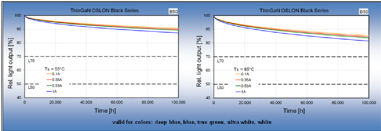
Figure 6: Degradation characteristics (*) of the OSLO Black Series with ThinGaN technology for T_s = 55^\circ\text{C} & T_s = 85^\circ\text{C} (grouping current I_F = 0.35\text{ A} )
