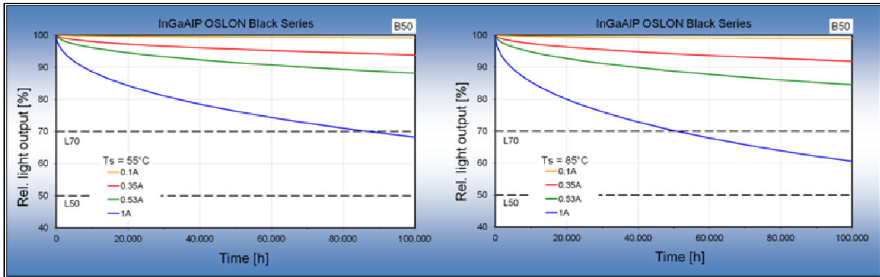
Figure 8: Degradation characteristics (*) of the OSLO Black Series with ThinFilm technology for T_s = 55^\circ\text{C} & T_s = 85^\circ\text{C} (grouping current I_F = 0.35\text{ A} )
