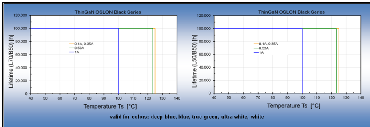
Figure 5: Lifetime (*) of the OSLOM Black Series with ThinGaN technology with respect to T_s
