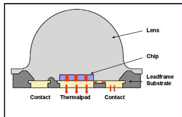
Figure 3: Primary heat flow in the OSOLON Black Series
