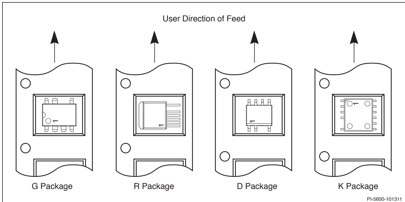
Figure 1. Part Orientation.
