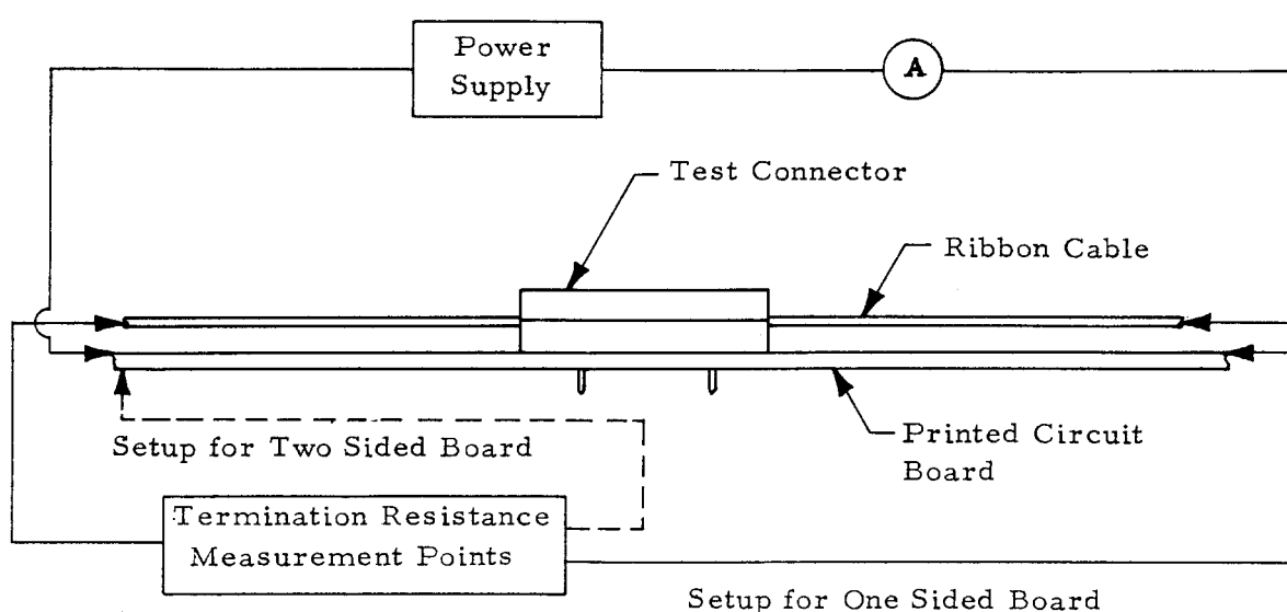
Figure 3 Termination Resistance Measurement Points
