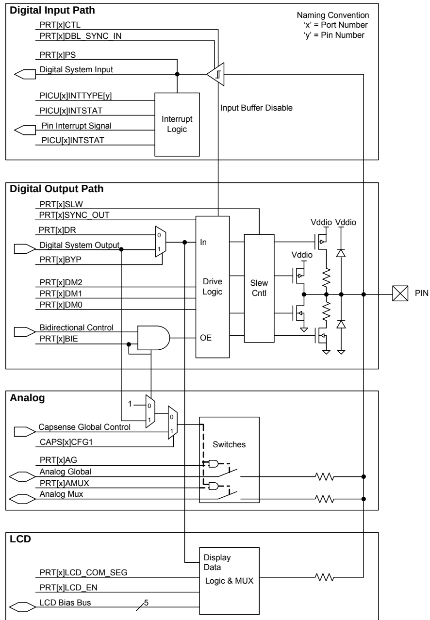
Figure 6-3.GPIO Block Diagram
