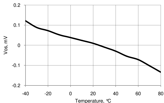
Figure 11-2. Opamp V_{os} vs Temperature, V_{DDA} = 5\text{ V}
