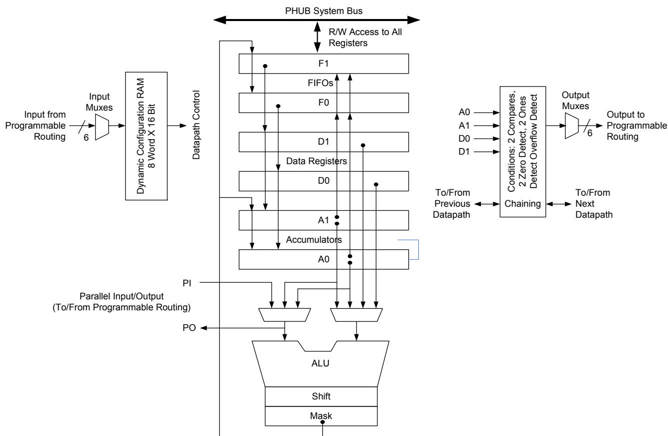
Figure 7-9.Datapath Top Level
