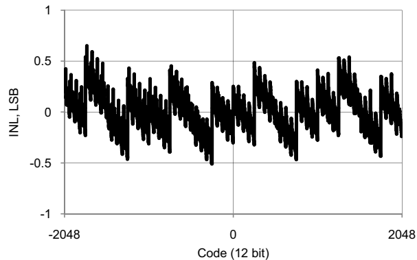
Figure 11-11. SAR ADC INL vs Output Code, Bypassed Internal Reference Mode
