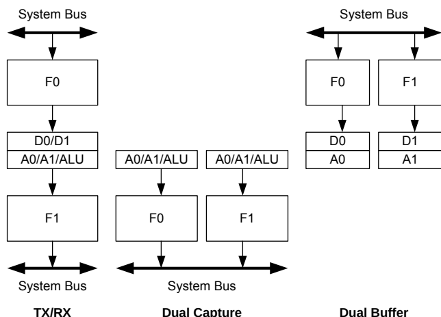
Figure 7-7.Example FIFO Configurations
