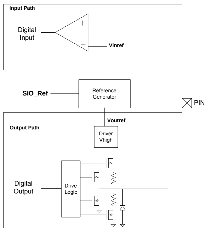
Figure 6-7. SIO Reference for Input and Output
