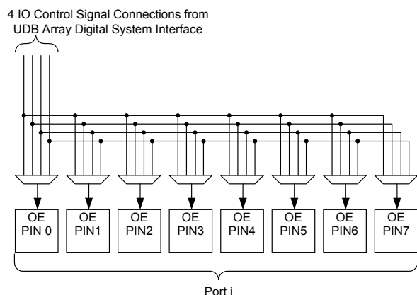
Figure 7-9. I/O Pin Output Enable Connectivity
