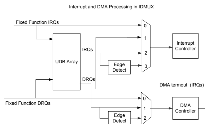
Figure 7-6. Interrupt and DMA Processing in the IDMUX
