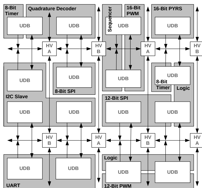
Figure 7-4. Function Mapping Example in a Bank of UDBs
