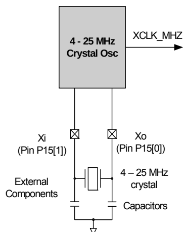
Figure 6-2.MHzECO Block Diagram
