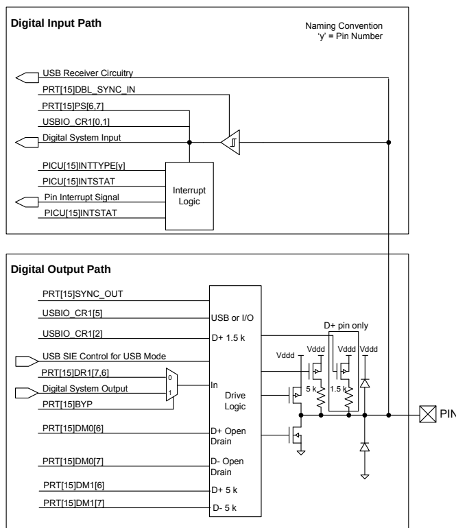
Figure 6-5.USBIO Block Diagram
