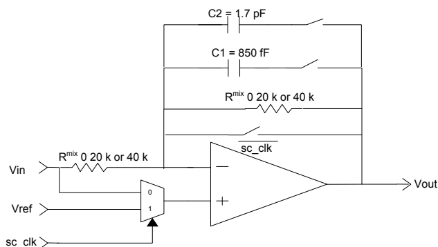
Figure 8-1.Mixer Configuration
