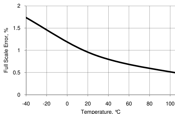
Figure 11-6.VDAC Full Scale Error vs Temperature, 4 V Mode
