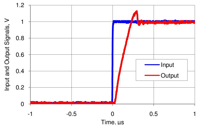
Figure 11-7. Opamp Step Response, Rising
