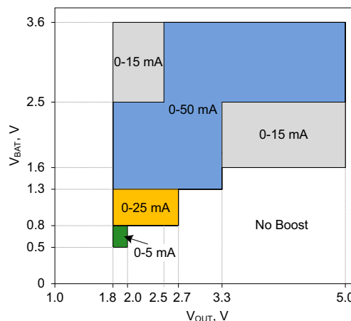
Figure 11-8. I_{\text{OUT}} range over V_{\text{BAT}} and V_{\text{OUT}}
