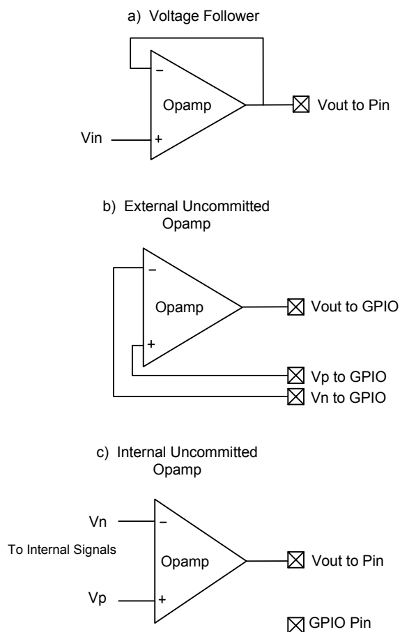
Figure 8-4.Opamp Configurations
