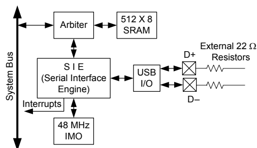
Figure 7-10. USB
