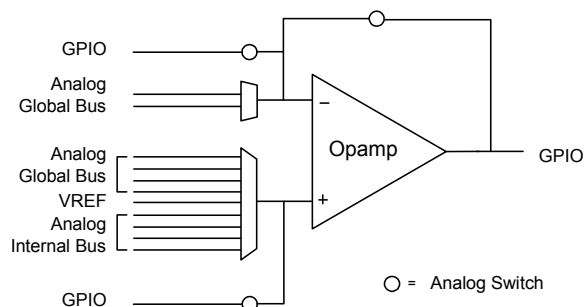
Figure 8-3.Opamp
