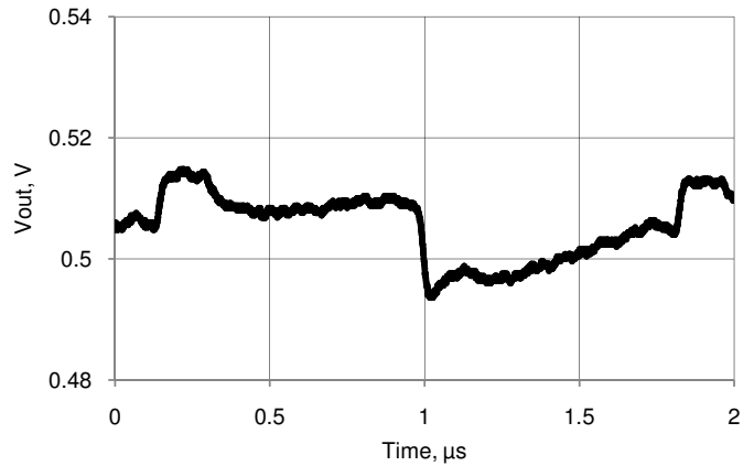
Figure 11-12.VDAC Voltage Noise, 1 V Mode, Fast Mode, V_{DDA} = 5 V
