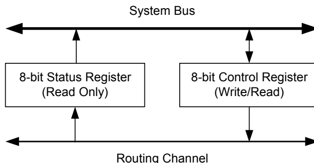
Figure 7-11.Status and Control Registers
