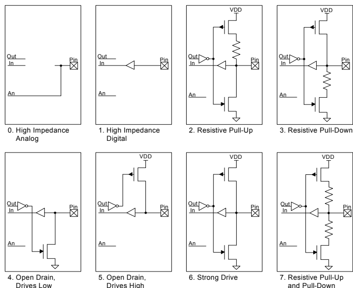
Figure 6-6. Drive Mode
