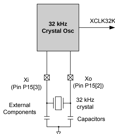
Figure 6-4.32kHzECO Block Diagram
