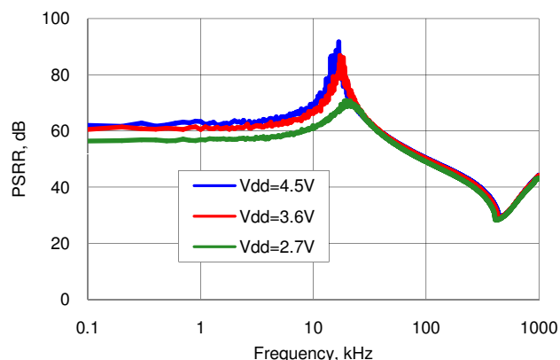
Figure 11-5. Digital Regulator PSRR vs Frequency and V_{DD}
