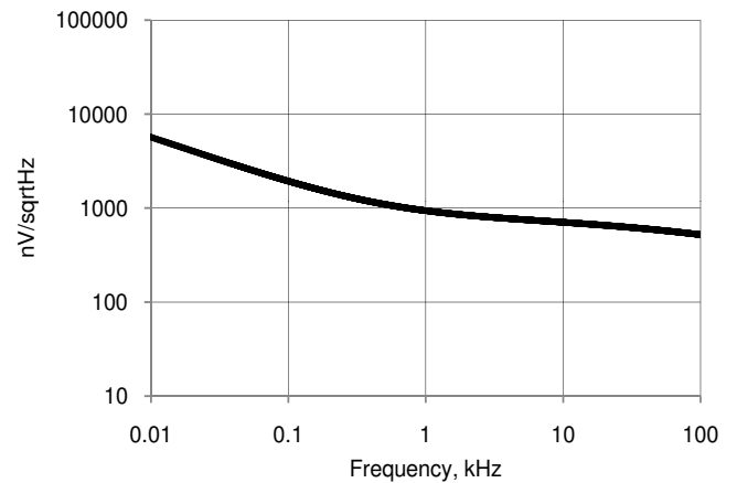
Figure 11-12.VDAC Voltage Noise, 1 V Mode, Fast Mode, V_{DDA} = 5 V
