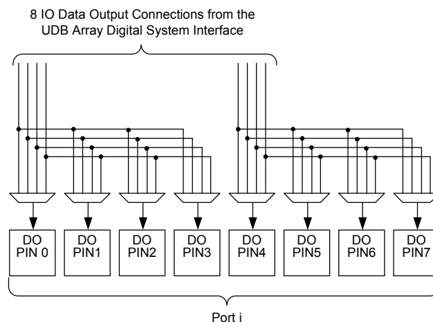
Figure 7-8. I/O Pin Output Connectivity
