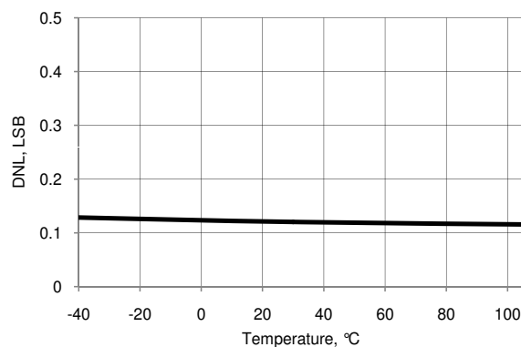
Figure 11-4.VDAC DNL vs Temperature, 1 V Mode
