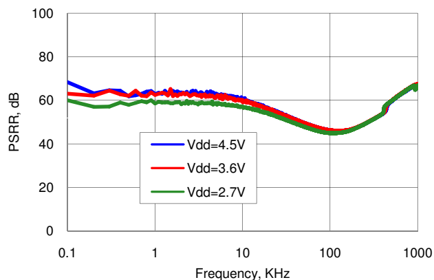
Figure 11-6. Analog Regulator PSRR vs Frequency and V_{DD}
