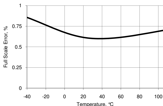
Figure 11-5.VDAC Full Scale Error vs Temperature, 1 V Mode
