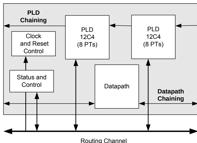
Figure 7-7.UDB Block Diagram
