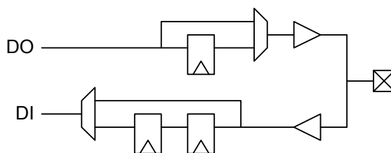
Figure 7-7. I/O Pin Synchronization Routing
