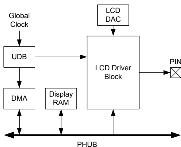
Figure 8-7. LCD System
