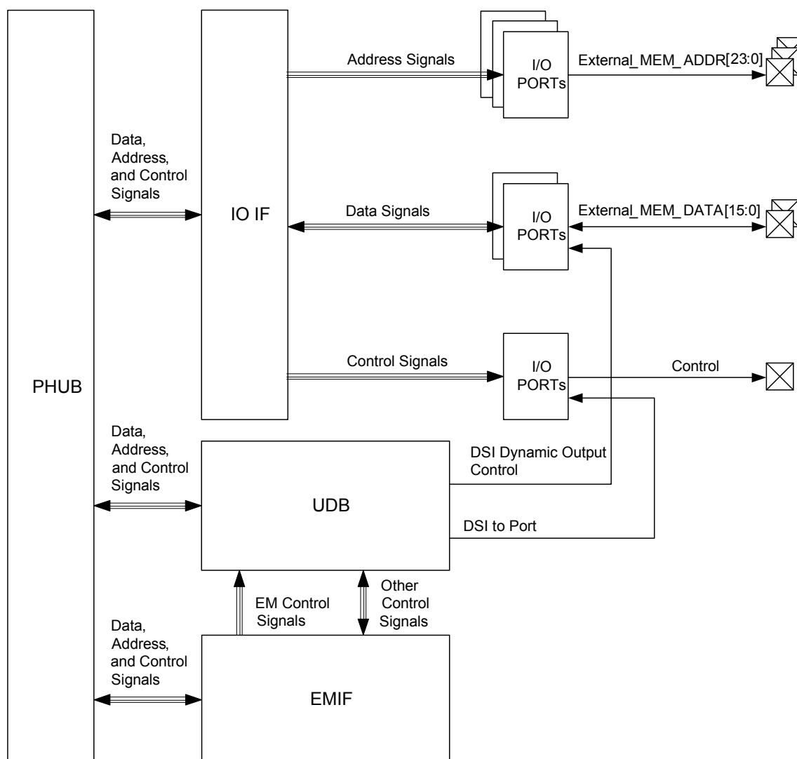
Figure 5-1.EMIF Block Diagram
