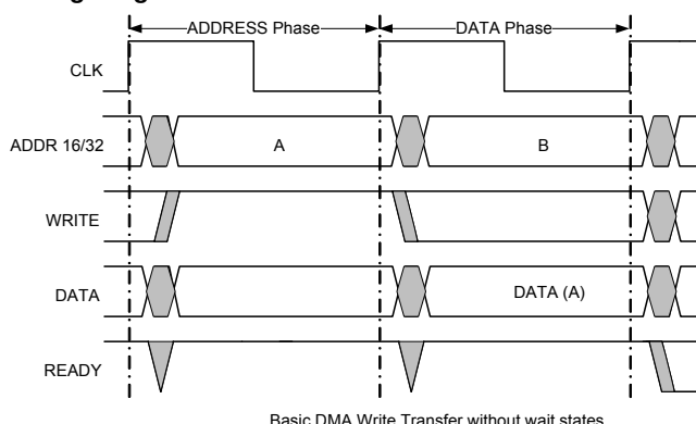
Figure 4-3. DMA Timing Diagram
