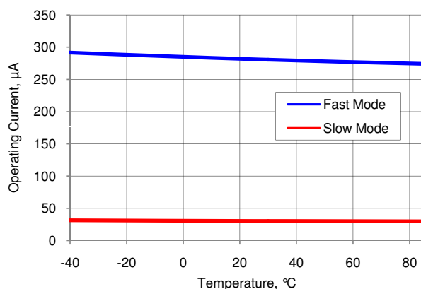
Figure 11-9.IDAC Operating Current vs Temperature, Range = 255 \mu A, Code = 0, Source Mode
