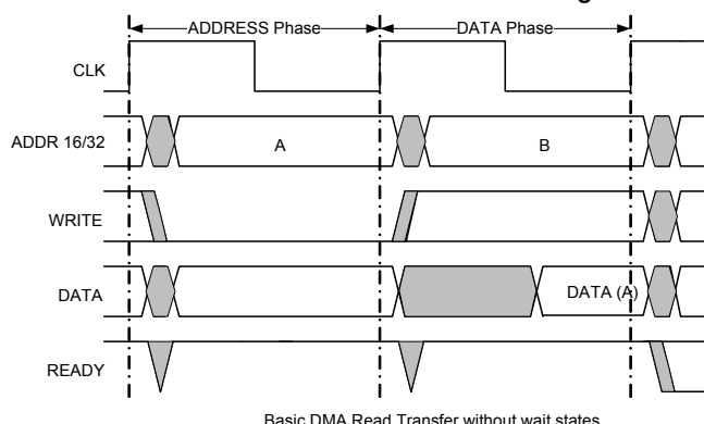
Figure 4-3. DMA Timing Diagram
