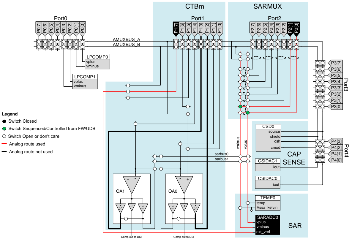
Figure 19-5. Input from External Pins
