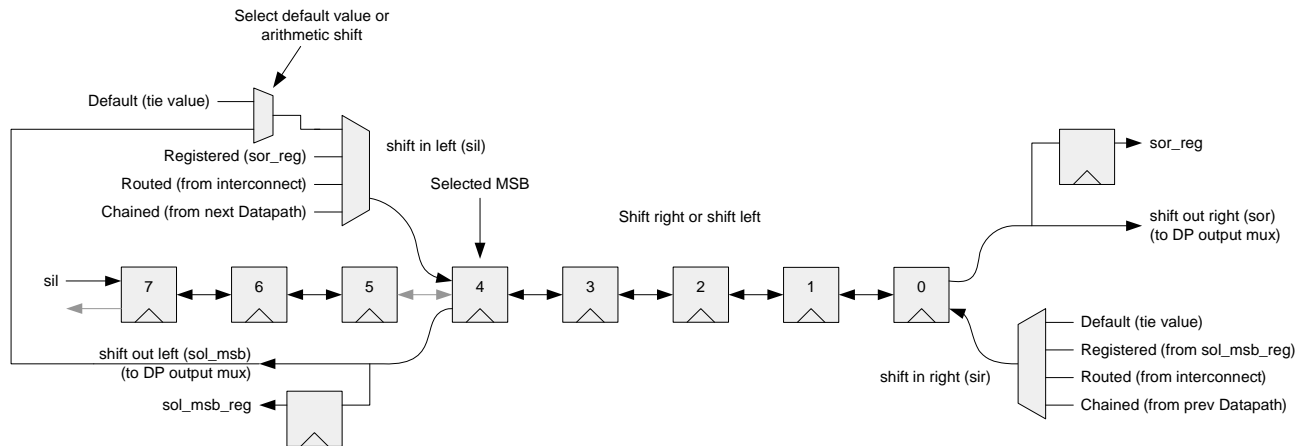
Figure 16-16. Shift Operation
