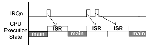
Figure 5-4. Pulse Interrupts
