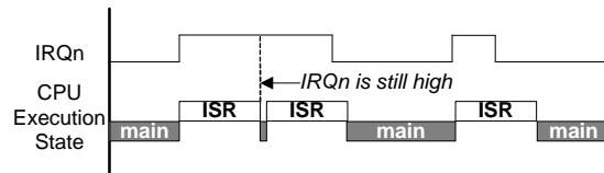
Figure 5-3. Level Interrupts
