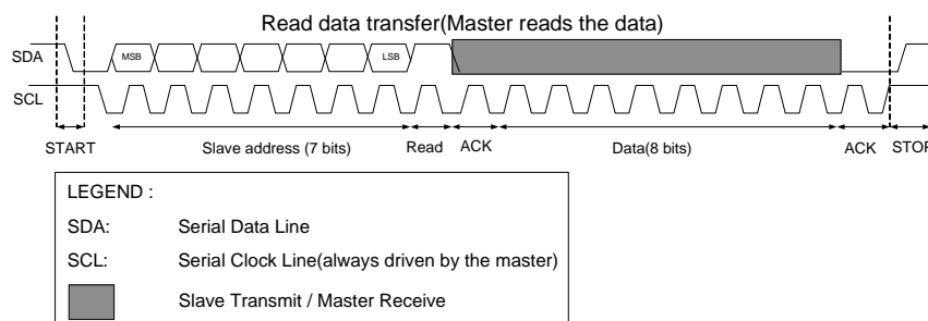
Figure 15-23. Master Read Data Transfer
