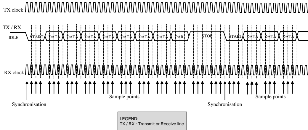
Figure 15-10. UART, Standard Protocol (Multiple Samples)
