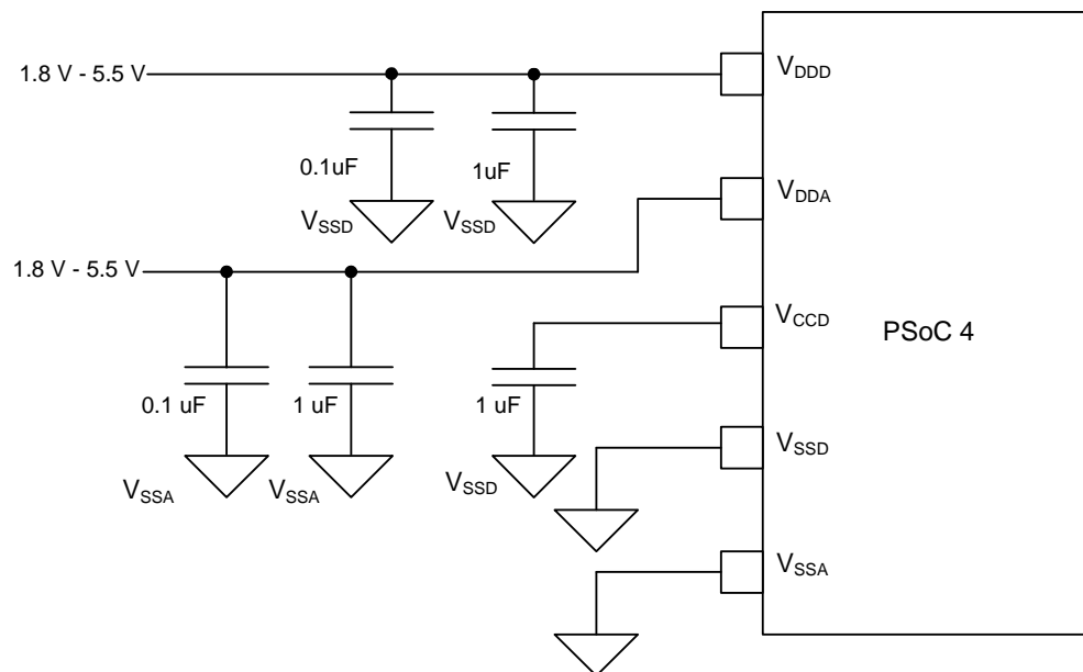
Figure 9-3. Separate Regulated V_{DDA} and V_{DD} Supplies
