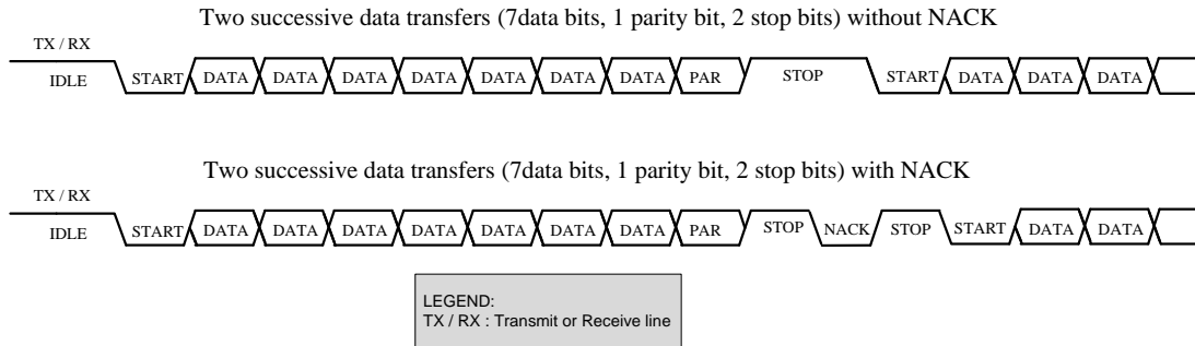
Figure 15-19. SmartCard Example
