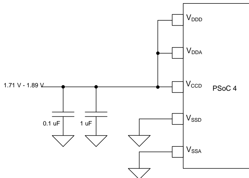
Figure 9-5. Single Unregulated Power Supply
