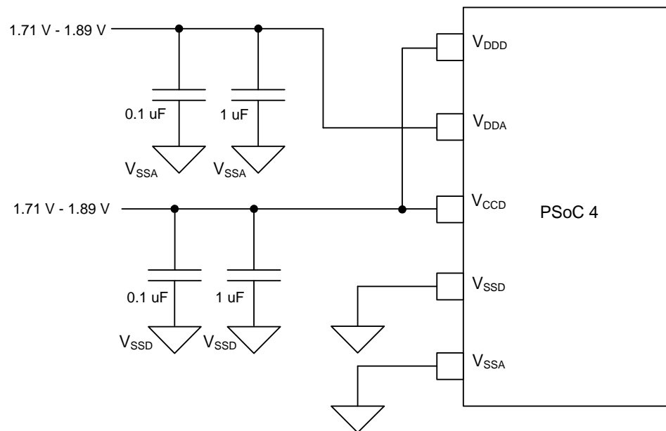
Figure 9-6. Separate Unregulated Power Supplies
