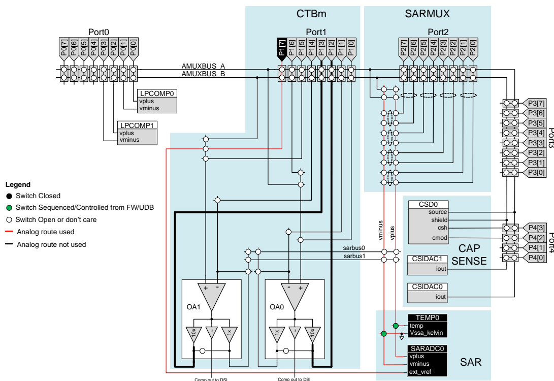
Figure 19-9. Inputs from Temperature Sensor
