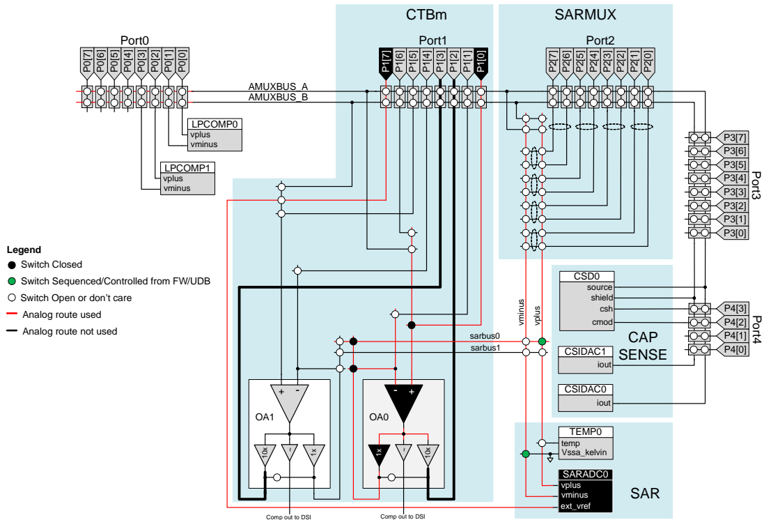
Figure 19-7. Input from CTBm Output via sarbus
