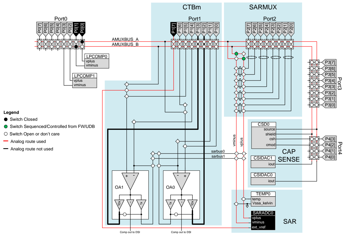
Figure 19-6. Input from Analog Bus
