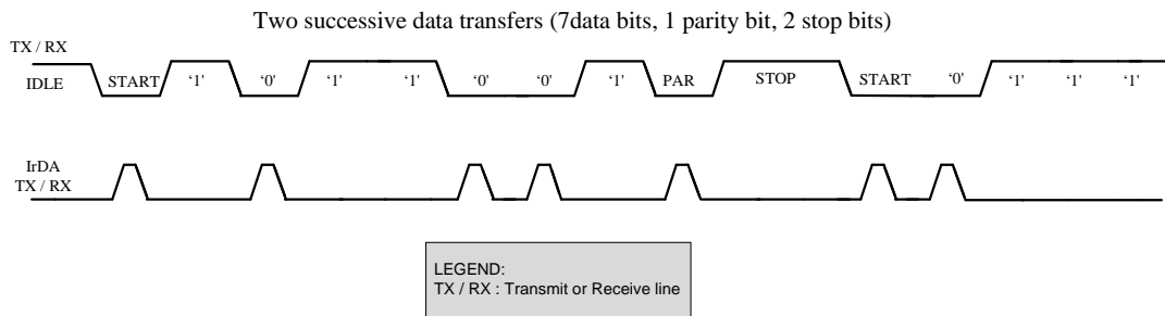
Figure 15-20. IrDA Example
