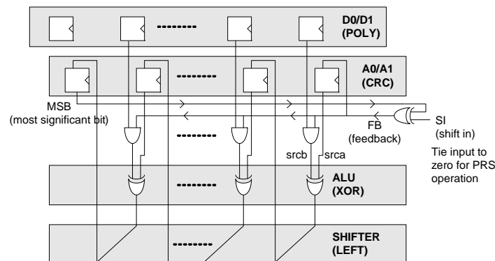
Figure 16-18. CRC Functional Structure
