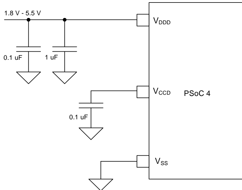
Figure 9-4. Single Regulated V_{DD} Supply
