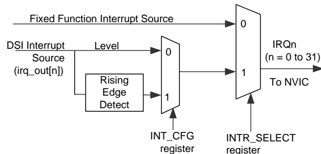
Figure 5-5. Interrupt Source Multiplexing
