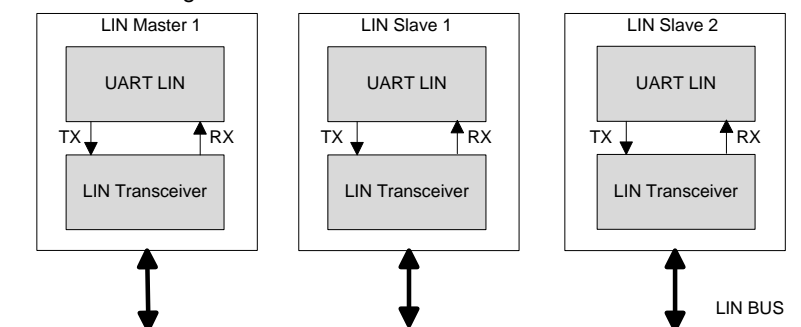
Figure 15-13. UART_LIN and LIN Transceiver
