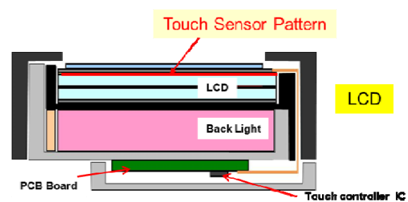
Fig. 2: On-Cell Touch technology
