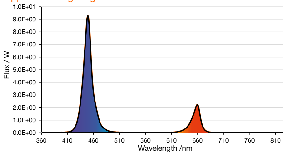
Figure 9: LED emission spectrum recommended for propagation by supplemental lighting
