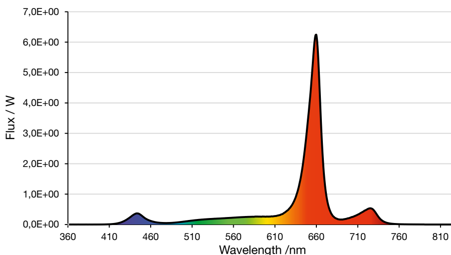
Figure 13: LED emission spectrum recommended for fruiting by supplemental lighting
