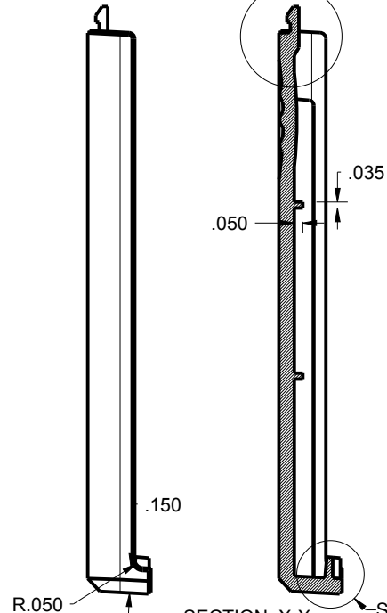
SECTION X-X
